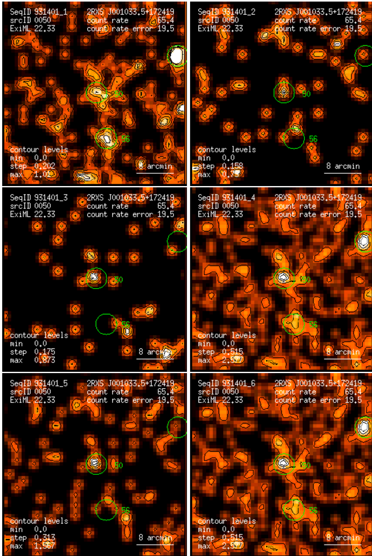
Figure 50: RASS 931401: detection 0050: band rate images, Gaussian filter: (1) PSPC channels 11 – 41, (2) 52 – 90, (3) 91 – 201, (4) 11 – 235, (5) 52 – 201, (6) 11 – 201. Broad band rates in counts/ks. Band rate contour levels in counts/ks/arcmin 2 .
