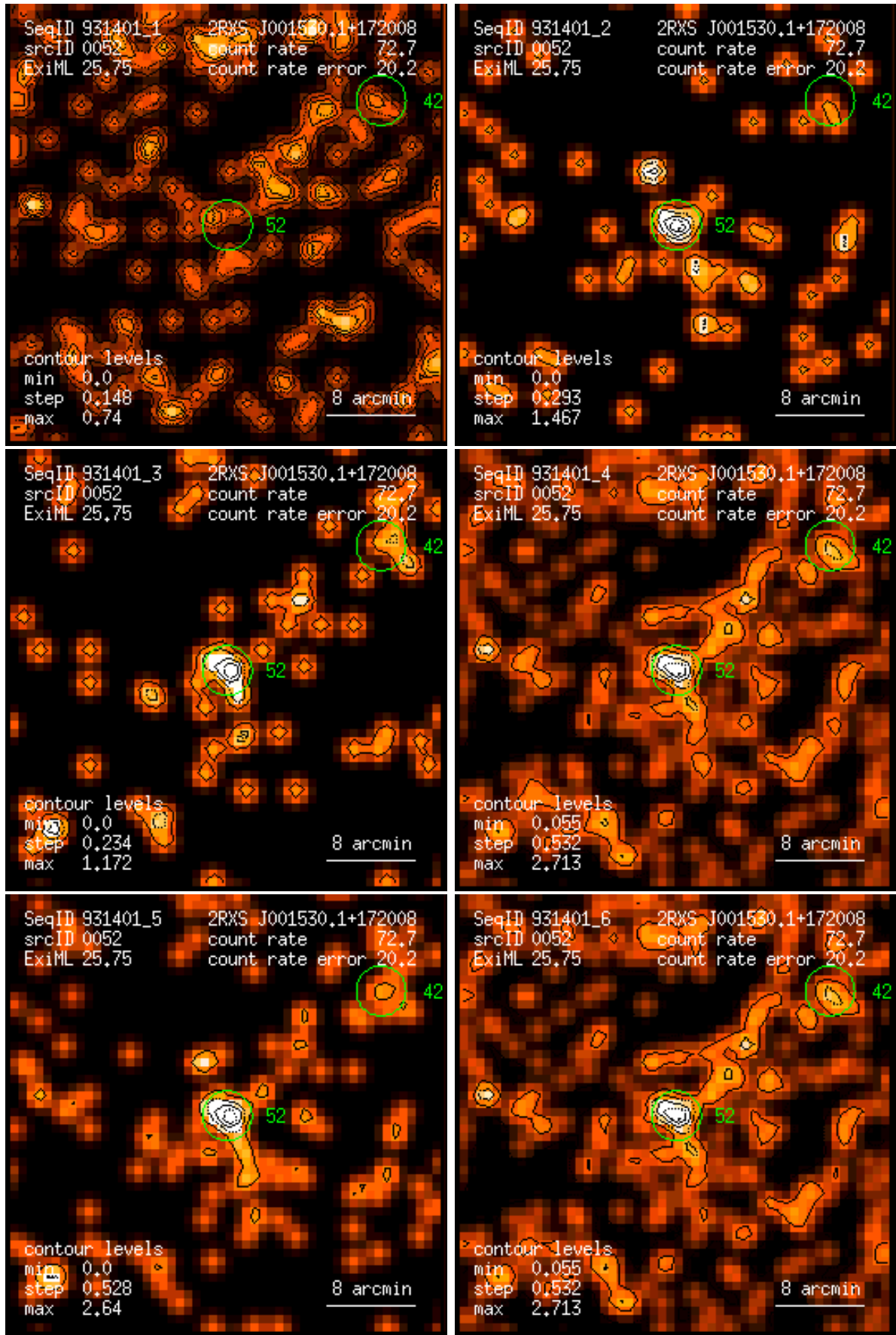
Figure 52: RASS 931401: detection 0052: band rate images, Gaussian filter: (1) PSPC channels 11 – 41, (2) 52 – 90, (3) 91 – 201, (4) 11 – 235, (5) 52 – 201, (6) 11 – 201. Broad band rates in counts/ks. Band rate contour levels in counts/ks/arcmin 2 .
