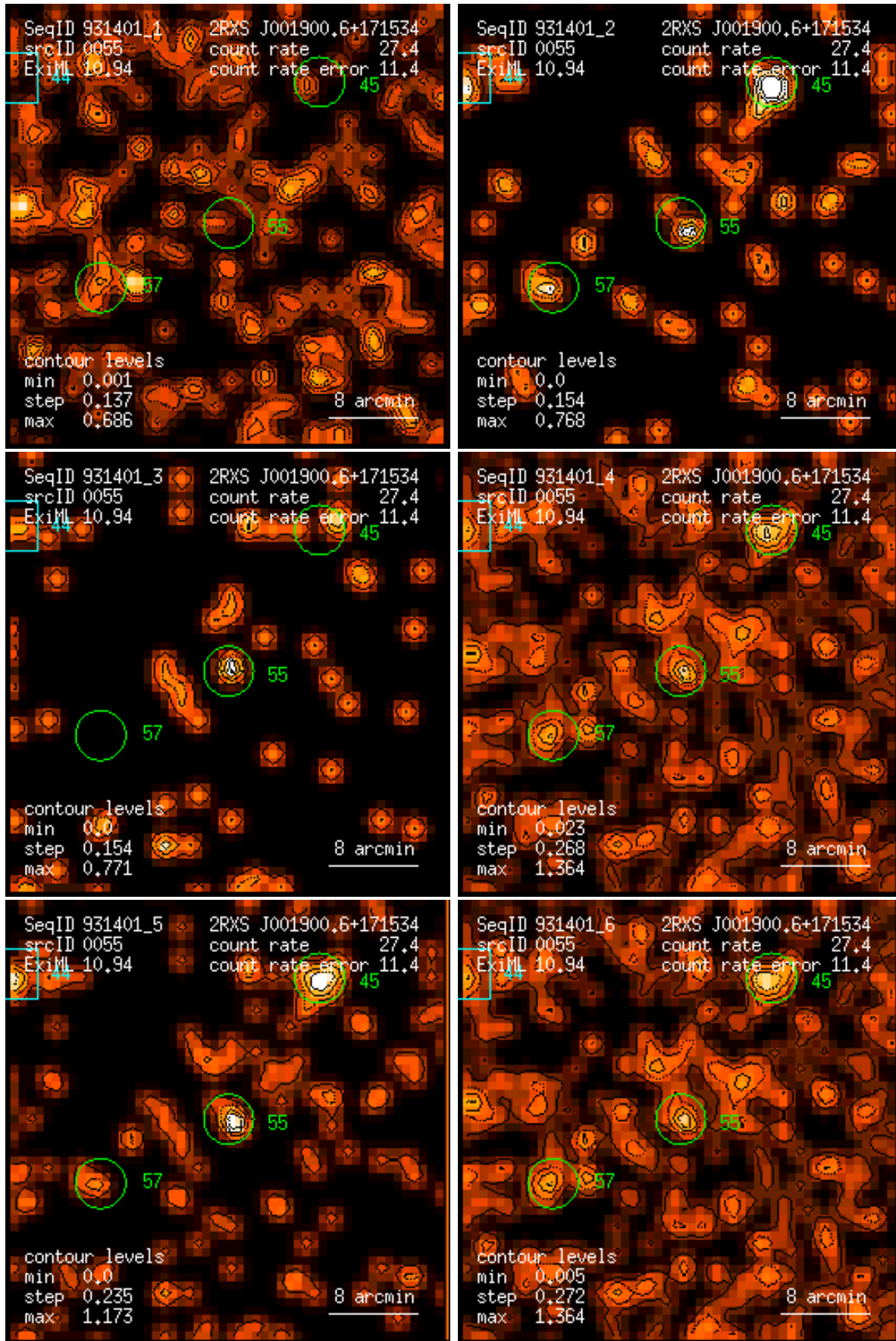
Figure 55: RASS 931401: detection 0055: band rate images, Gaussian filter: (1) PSPC channels 11 – 41, (2) 52 – 90, (3) 91 – 201, (4) 11 – 235, (5) 52 – 201, (6) 11 – 201. Broad band rates in counts/ks. Band rate contour levels in counts/ks/arcmin 2 .
