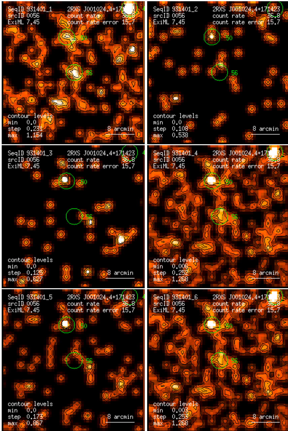
Figure 56: RASS 931401: detection 0056: band rate images, Gaussian filter: (1) PSPC channels 11 – 41, (2) 52 – 90, (3) 91 – 201, (4) 11 – 235, (5) 52 – 201, (6) 11 – 201. Broad band rates in counts/ks. Band rate contour levels in counts/ks/arcmin 2 .
