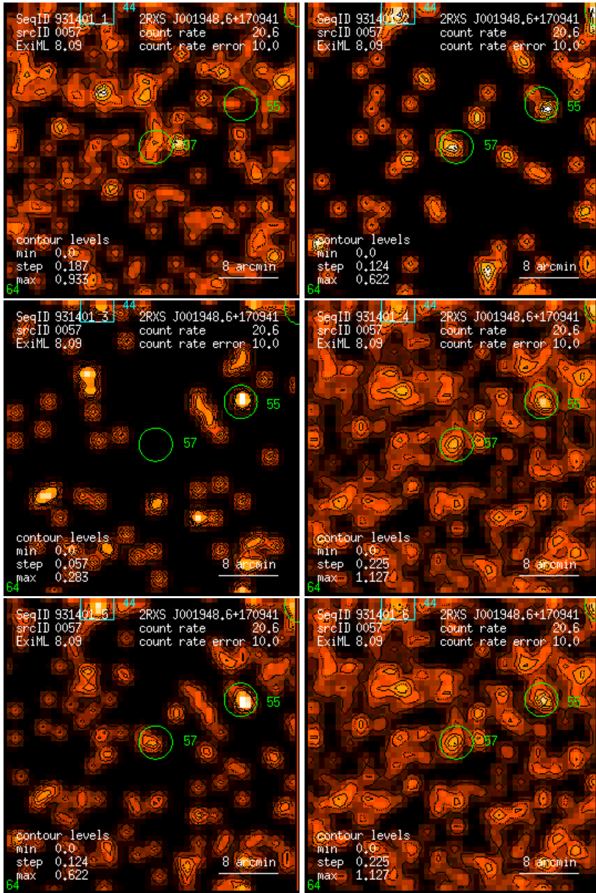
Figure 57: RASS 931401: detection 0057: band rate images, Gaussian filter: (1) PSPC channels 11 – 41, (2) 52 – 90, (3) 91 – 201, (4) 11 – 235, (5) 52 – 201, (6) 11 – 201. Broad band rates in counts/ks. Band rate contour levels in counts/ks/arcmin 2 .
