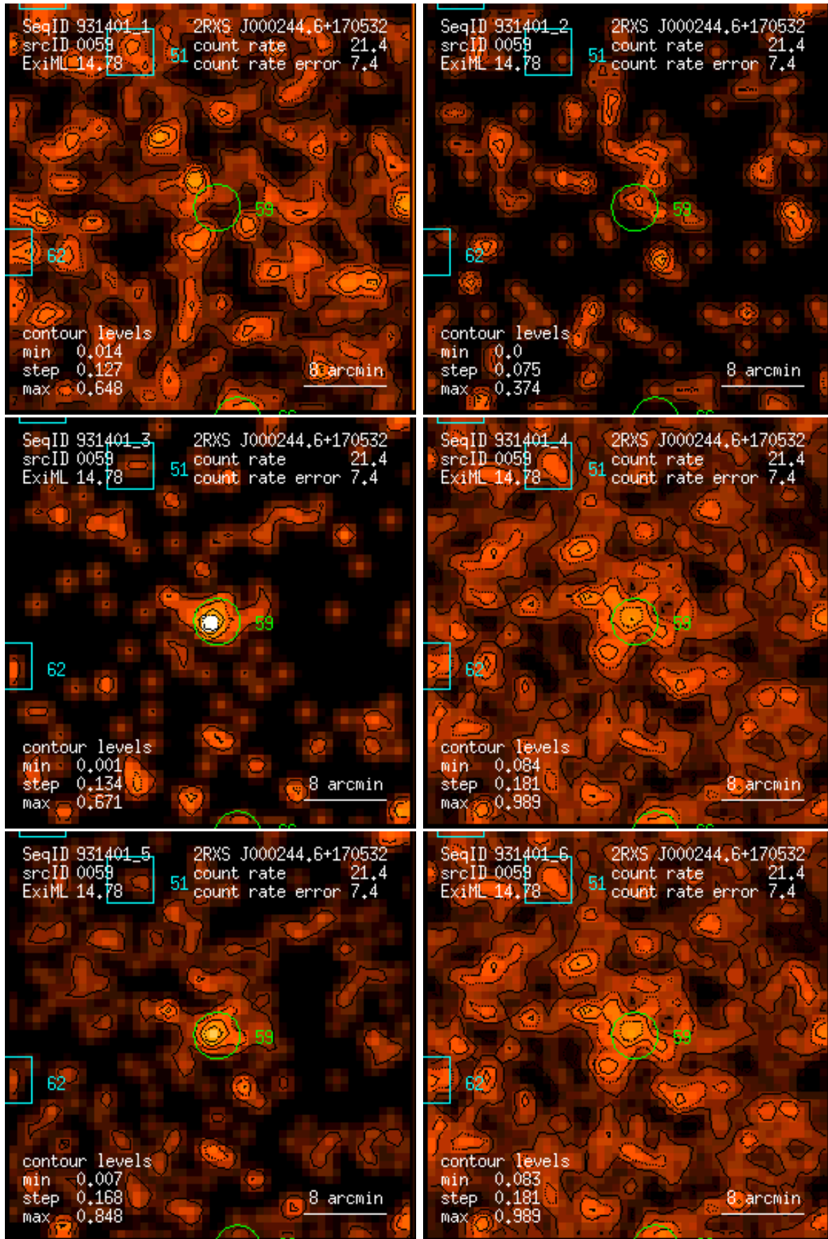
Figure 59: RASS 931401: detection 0059: band rate images, Gaussian filter: (1) PSPC channels 11 – 41, (2) 52 – 90, (3) 91 – 201, (4) 11 – 235, (5) 52 – 201, (6) 11 – 201. Broad band rates in counts/ks. Band rate contour levels in counts/ks/arcmin 2 .
