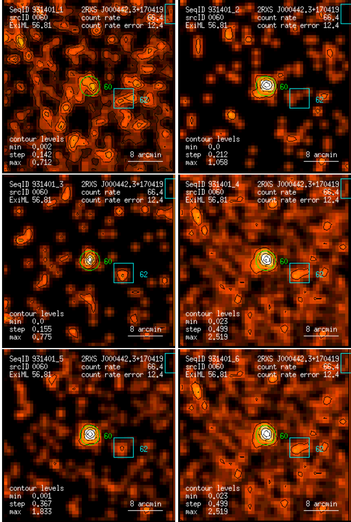
Figure 60: RASS 931401: detection 0060: band rate images, Gaussian filter: (1) PSPC channels 11 – 41, (2) 52 – 90, (3) 91 – 201, (4) 11 – 235, (5) 52 – 201, (6) 11 – 201. Broad band rates in counts/ks. Band rate contour levels in counts/ks/arcmin 2 .
