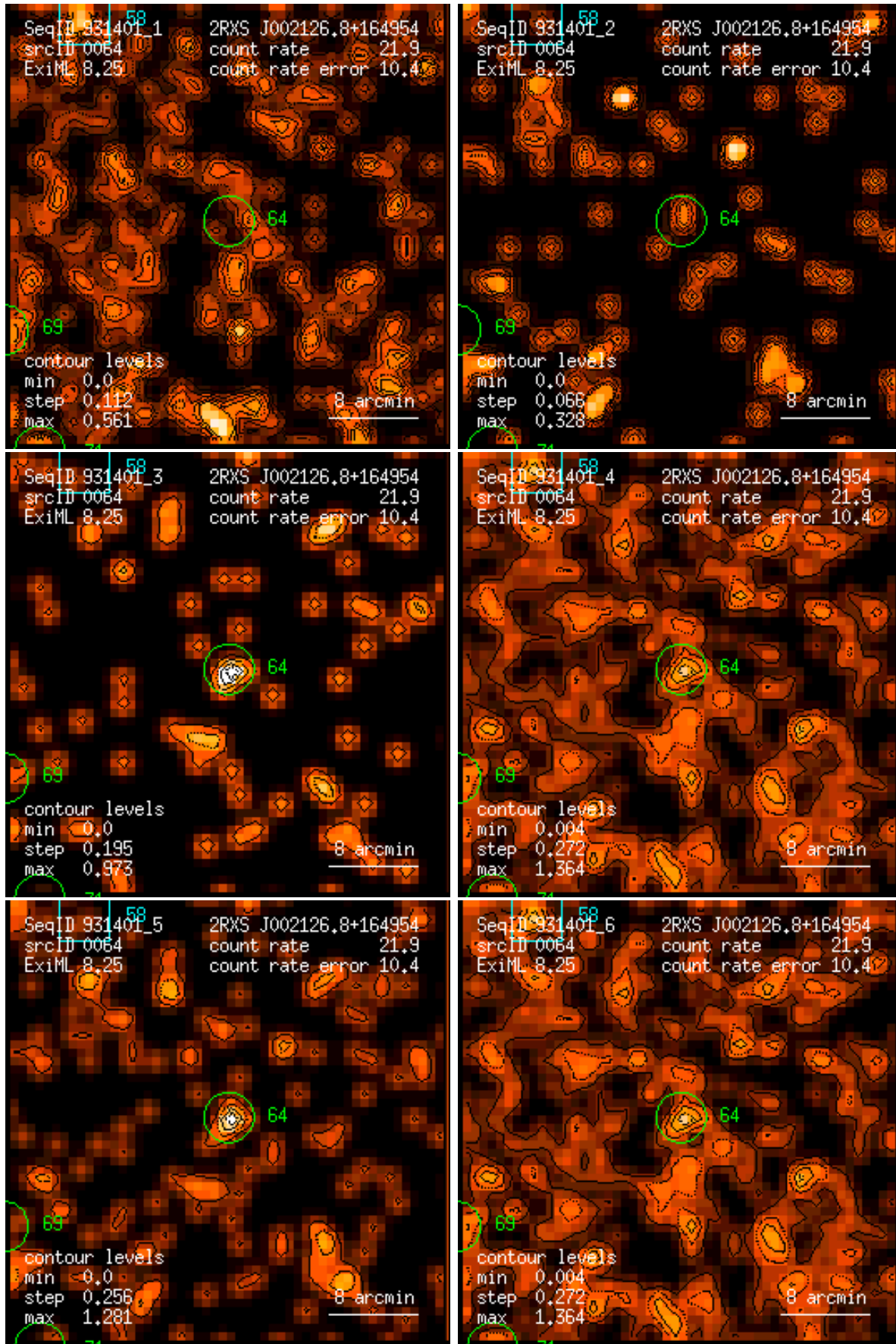
Figure 64: RASS 931401: detection 0064: band rate images, Gaussian filter: (1) PSPC channels 11 – 41, (2) 52 – 90, (3) 91 – 201, (4) 11 – 235, (5) 52 – 201, (6) 11 – 201. Broad band rates in counts/ks. Band rate contour levels in counts/ks/arcmin 2 .
