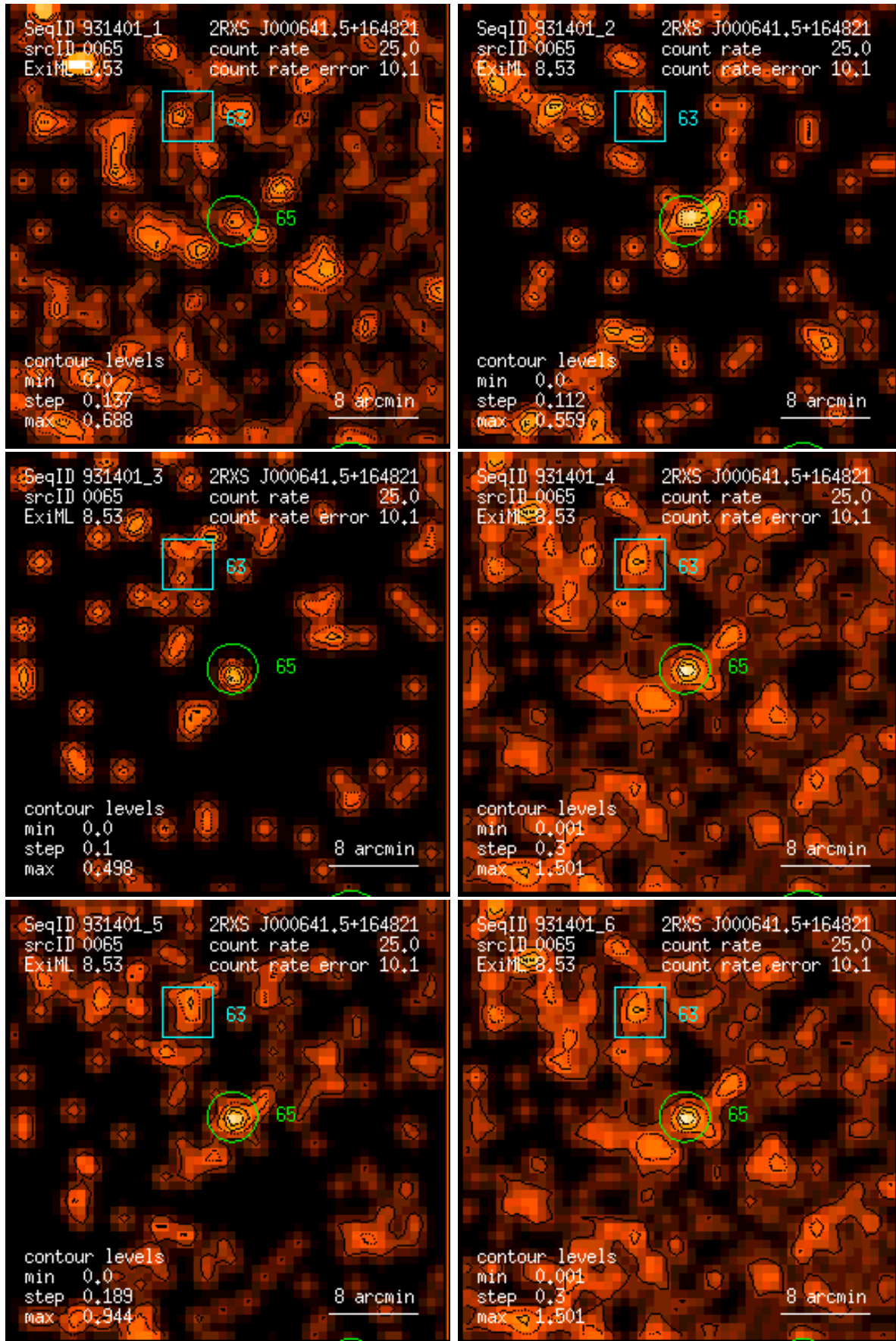
Figure 65: RASS 931401: detection 0065: band rate images, Gaussian filter: (1) PSPC channels 11 – 41, (2) 52 – 90, (3) 91 – 201, (4) 11 – 235, (5) 52 – 201, (6) 11 – 201. Broad band rates in counts/ks. Band rate contour levels in counts/ks/arcmin 2 .
