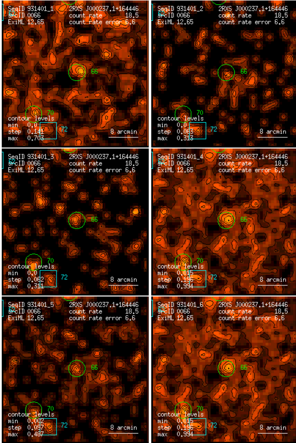
Figure 66: RASS 931401: detection 0066: band rate images, Gaussian filter: (1) PSPC channels 11 – 41, (2) 52 – 90, (3) 91 – 201, (4) 11 – 235, (5) 52 – 201, (6) 11 – 201. Broad band rates in counts/ks. Band rate contour levels in counts/ks/arcmin 2 .
