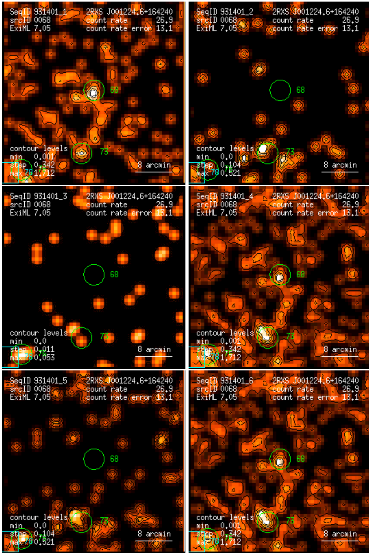
Figure 68: RASS 931401: detection 0068: band rate images, Gaussian filter: (1) PSPC channels 11 – 41, (2) 52 – 90, (3) 91 – 201, (4) 11 – 235, (5) 52 – 201, (6) 11 – 201. Broad band rates in counts/ks. Band rate contour levels in counts/ks/arcmin 2 .
