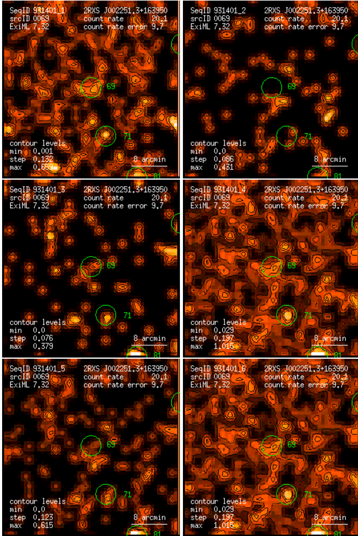
Figure 69: RASS 931401: detection 0069: band rate images, Gaussian filter: (1) PSPC channels 11 – 41, (2) 52 – 90, (3) 91 – 201, (4) 11 – 235, (5) 52 – 201, (6) 11 – 201. Broad band rates in counts/ks. Band rate contour levels in counts/ks/arcmin 2 .
