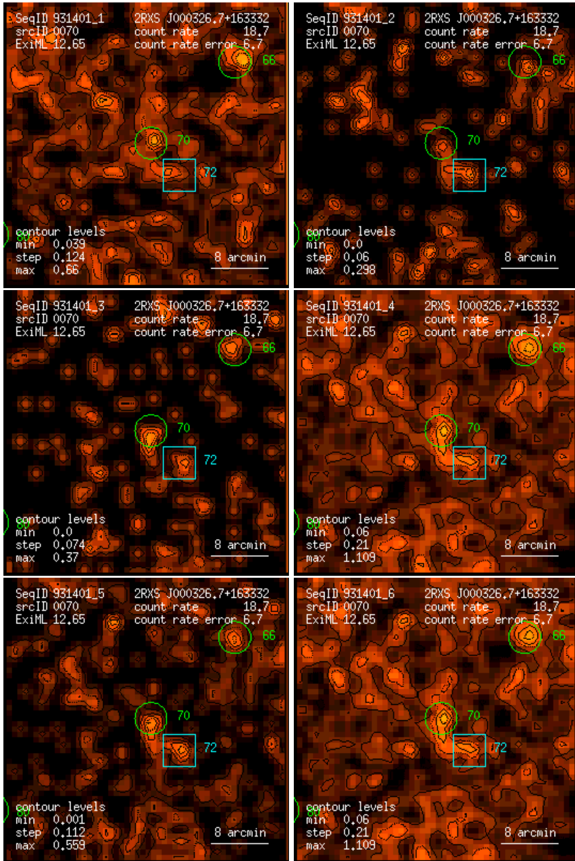
Figure 70: RASS 931401: detection 0070: band rate images, Gaussian filter: (1) PSPC channels 11 – 41, (2) 52 – 90, (3) 91 – 201, (4) 11 – 235, (5) 52 – 201, (6) 11 – 201. Broad band rates in counts/ks. Band rate contour levels in counts/ks/arcmin 2 .
