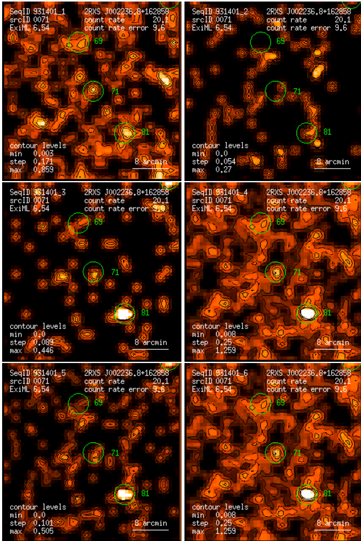
Figure 71: RASS 931401: detection 0071: band rate images, Gaussian filter: (1) PSPC channels 11 – 41, (2) 52 – 90, (3) 91 – 201, (4) 11 – 235, (5) 52 – 201, (6) 11 – 201. Broad band rates in counts/ks. Band rate contour levels in counts/ks/arcmin 2 .
