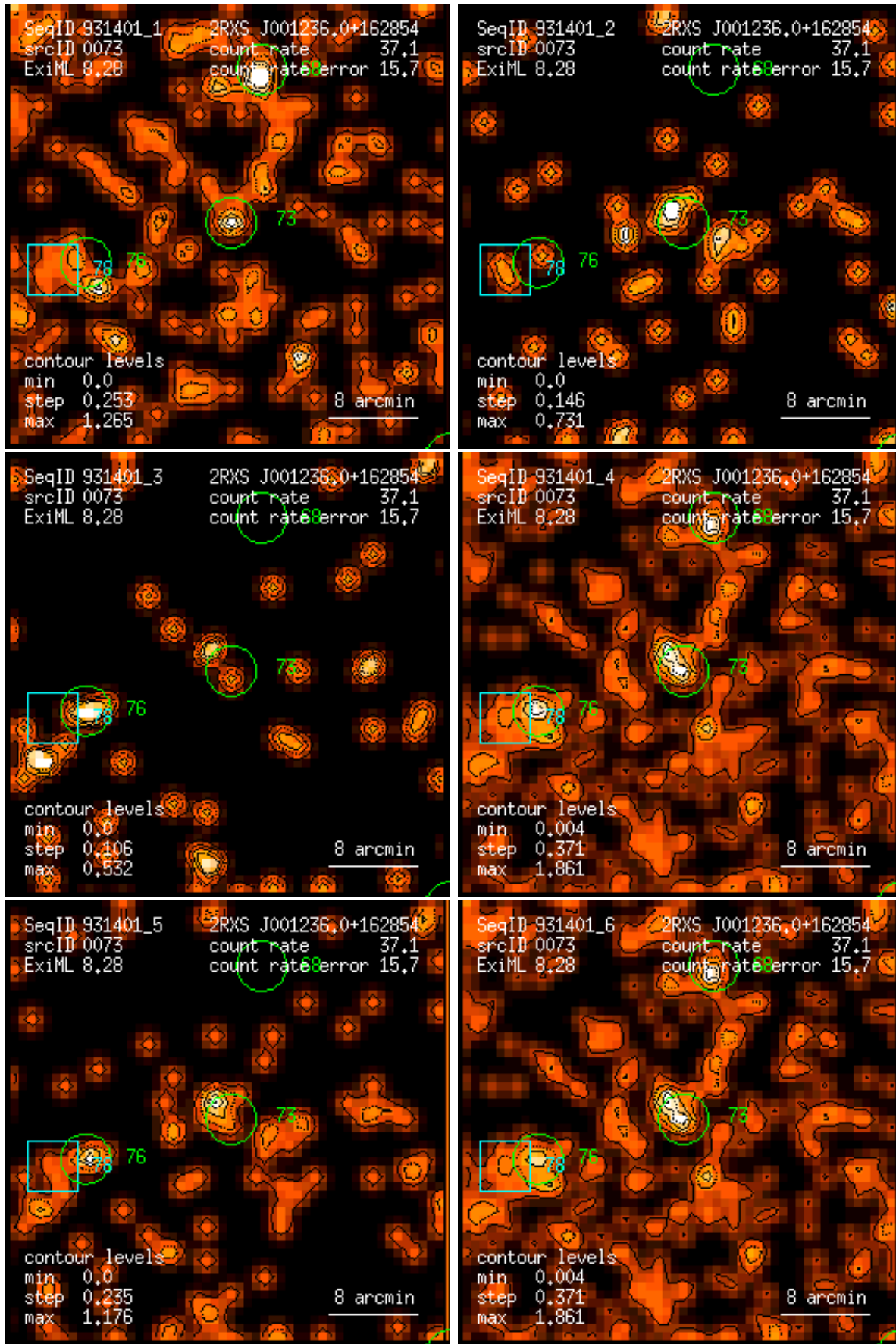
Figure 73: RASS 931401: detection 0073: band rate images, Gaussian filter: (1) PSPC channels 11 – 41, (2) 52 – 90, (3) 91 – 201, (4) 11 – 235, (5) 52 – 201, (6) 11 – 201. Broad band rates in counts/ks. Band rate contour levels in counts/ks/arcmin 2 .
