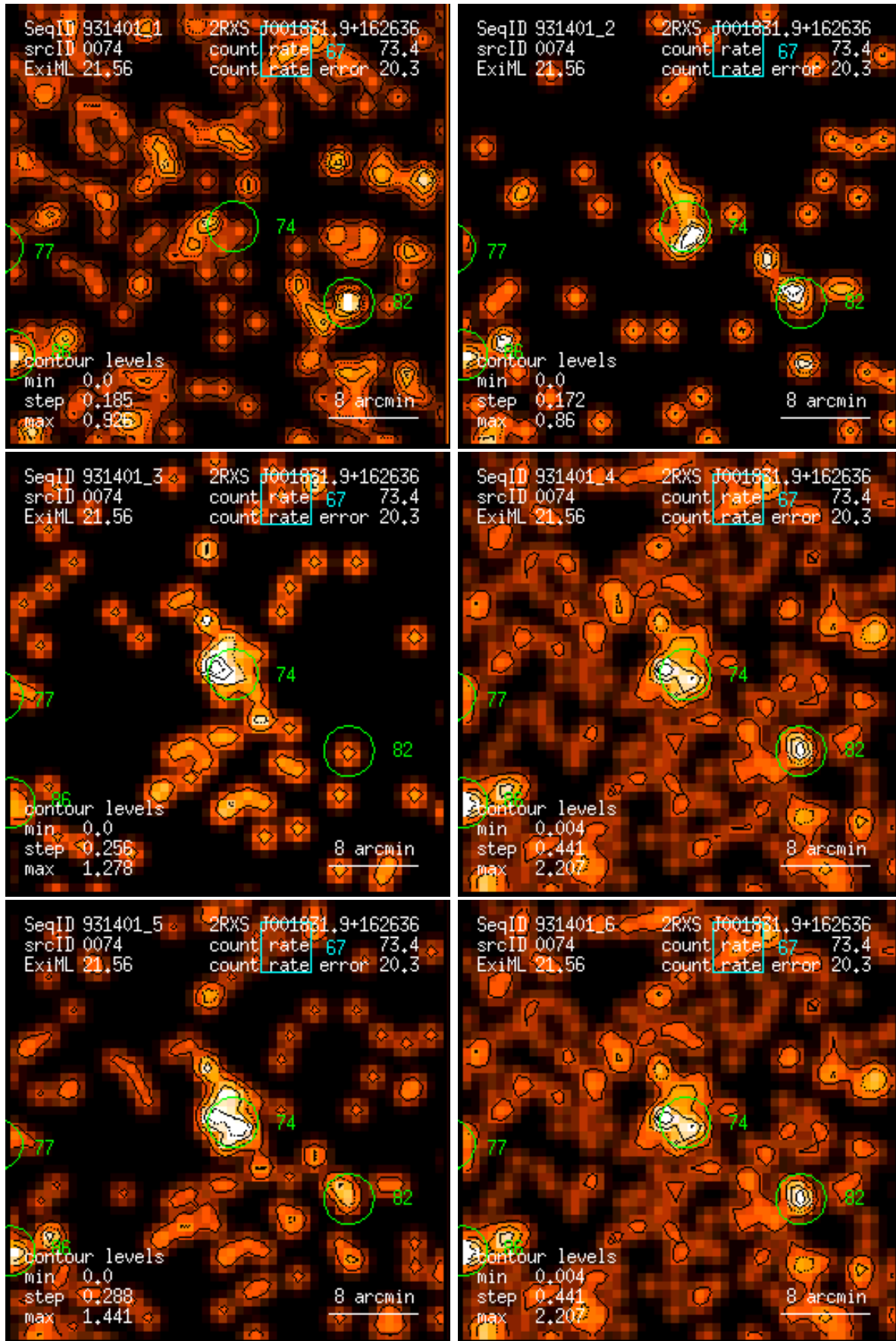
Figure 74: RASS 931401: detection 0074: band rate images, Gaussian filter: (1) PSPC channels 11 – 41, (2) 52 – 90, (3) 91 – 201, (4) 11 – 235, (5) 52 – 201, (6) 11 – 201. Broad band rates in counts/ks. Band rate contour levels in counts/ks/arcmin 2 .
