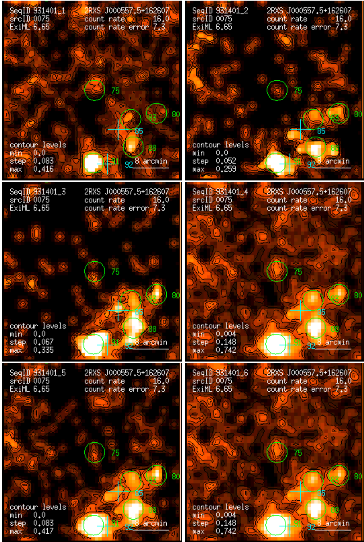
Figure 75: RASS 931401: detection 0075: band rate images, Gaussian filter: (1) PSPC channels 11 – 41, (2) 52 – 90, (3) 91 – 201, (4) 11 – 235, (5) 52 – 201, (6) 11 – 201. Broad band rates in counts/ks. Band rate contour levels in counts/ks/arcmin 2 .
