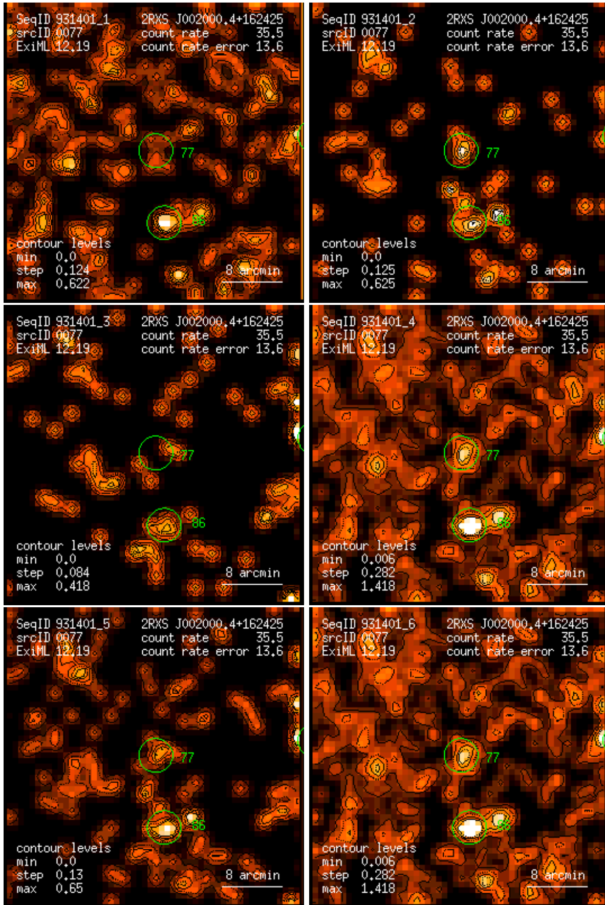
Figure 77: RASS 931401: detection 0077: band rate images, Gaussian filter: (1) PSPC channels 11 – 41, (2) 52 – 90, (3) 91 – 201, (4) 11 – 235, (5) 52 – 201, (6) 11 – 201. Broad band rates in counts/ks. Band rate contour levels in counts/ks/arcmin 2 .
