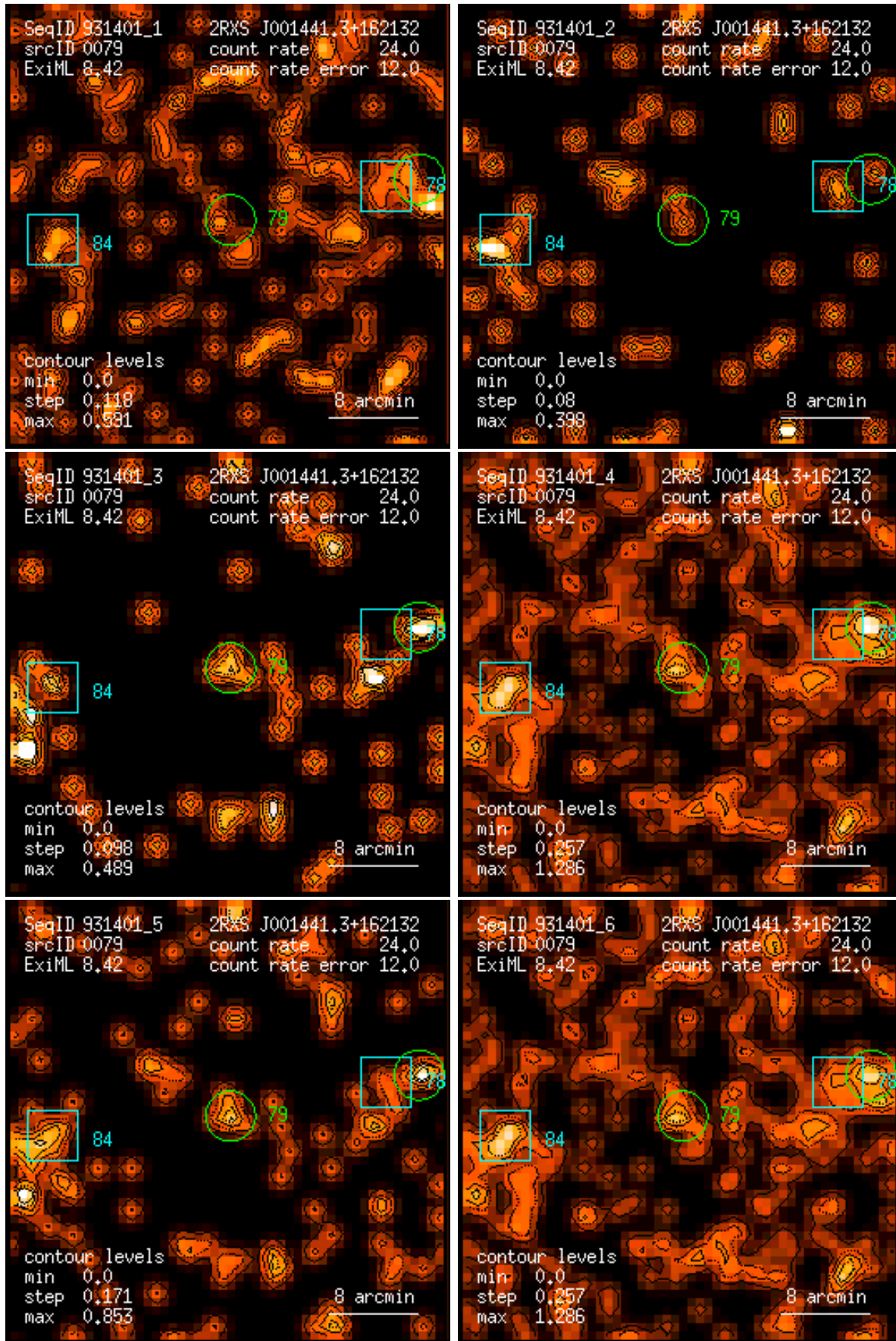
Figure 79: RASS 931401: detection 0079: band rate images, Gaussian filter: (1) PSPC channels 11 – 41, (2) 52 – 90, (3) 91 – 201, (4) 11 – 235, (5) 52 – 201, (6) 11 – 201. Broad band rates in counts/ks. Band rate contour levels in counts/ks/arcmin 2 .
