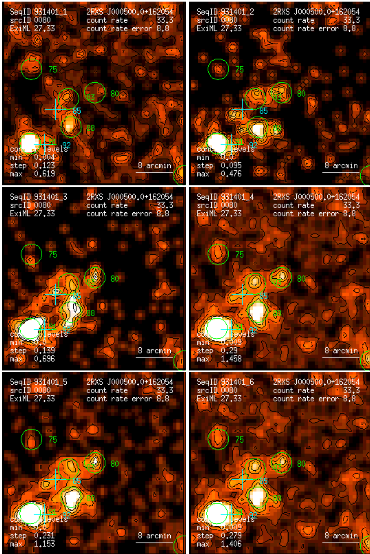
Figure 80: RASS 931401: detection 0080: band rate images, Gaussian filter: (1) PSPC channels 11 – 41, (2) 52 – 90, (3) 91 – 201, (4) 11 – 235, (5) 52 – 201, (6) 11 – 201. Broad band rates in counts/ks. Band rate contour levels in counts/ks/arcmin 2 .
