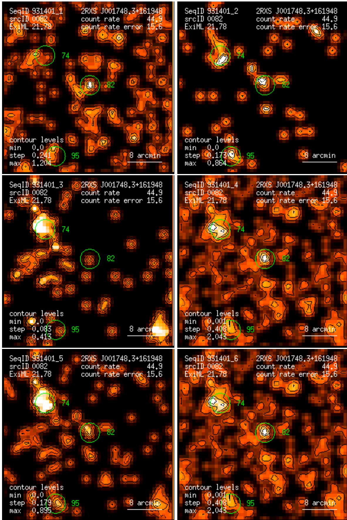
Figure 82: RASS 931401: detection 0082: band rate images, Gaussian filter: (1) PSPC channels 11 – 41, (2) 52 – 90, (3) 91 – 201, (4) 11 – 235, (5) 52 – 201, (6) 11 – 201. Broad band rates in counts/ks. Band rate contour levels in counts/ks/arcmin 2 .
