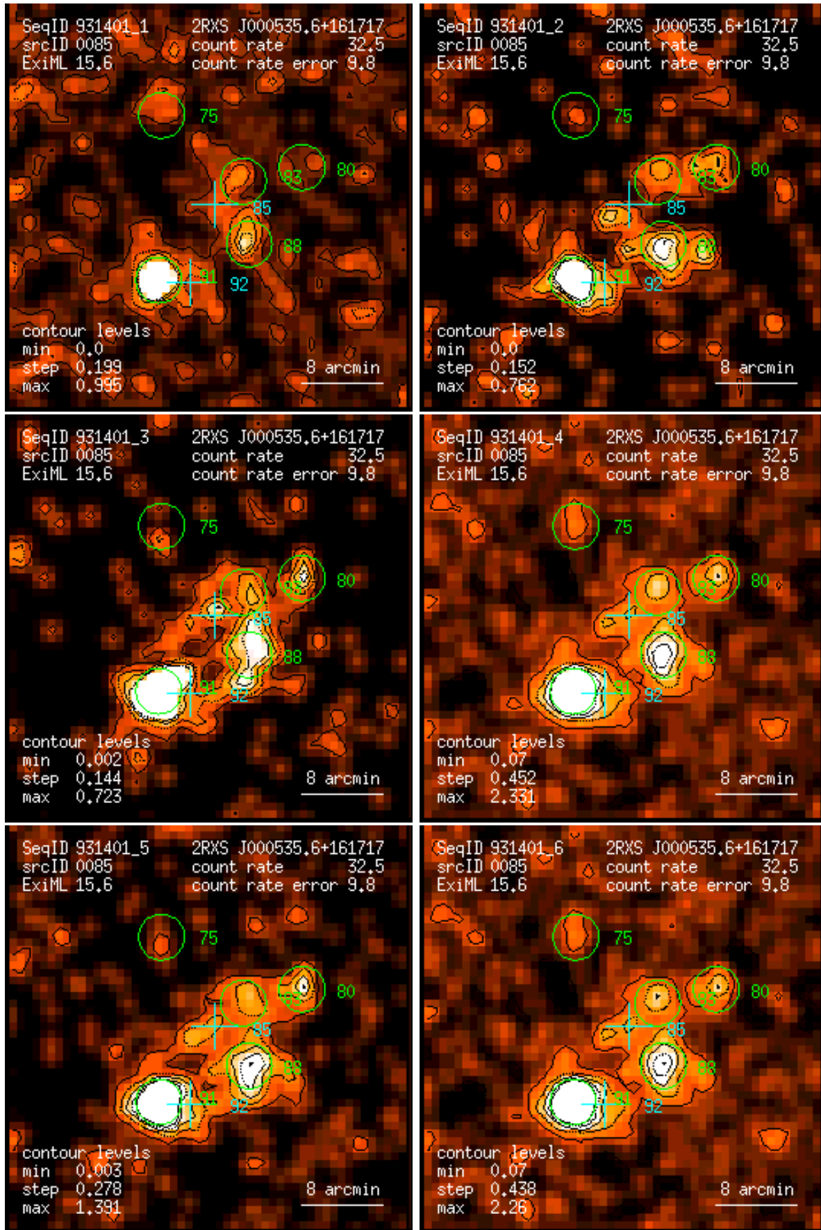
Figure 85: RASS 931401: detection 0085: band rate images, Gaussian filter: (1) PSPC channels 11 – 41, (2) 52 – 90, (3) 91 – 201, (4) 11 – 235, (5) 52 – 201, (6) 11 – 201. Broad band rates in counts/ks. Band rate contour levels in counts/ks/arcmin 2 .
