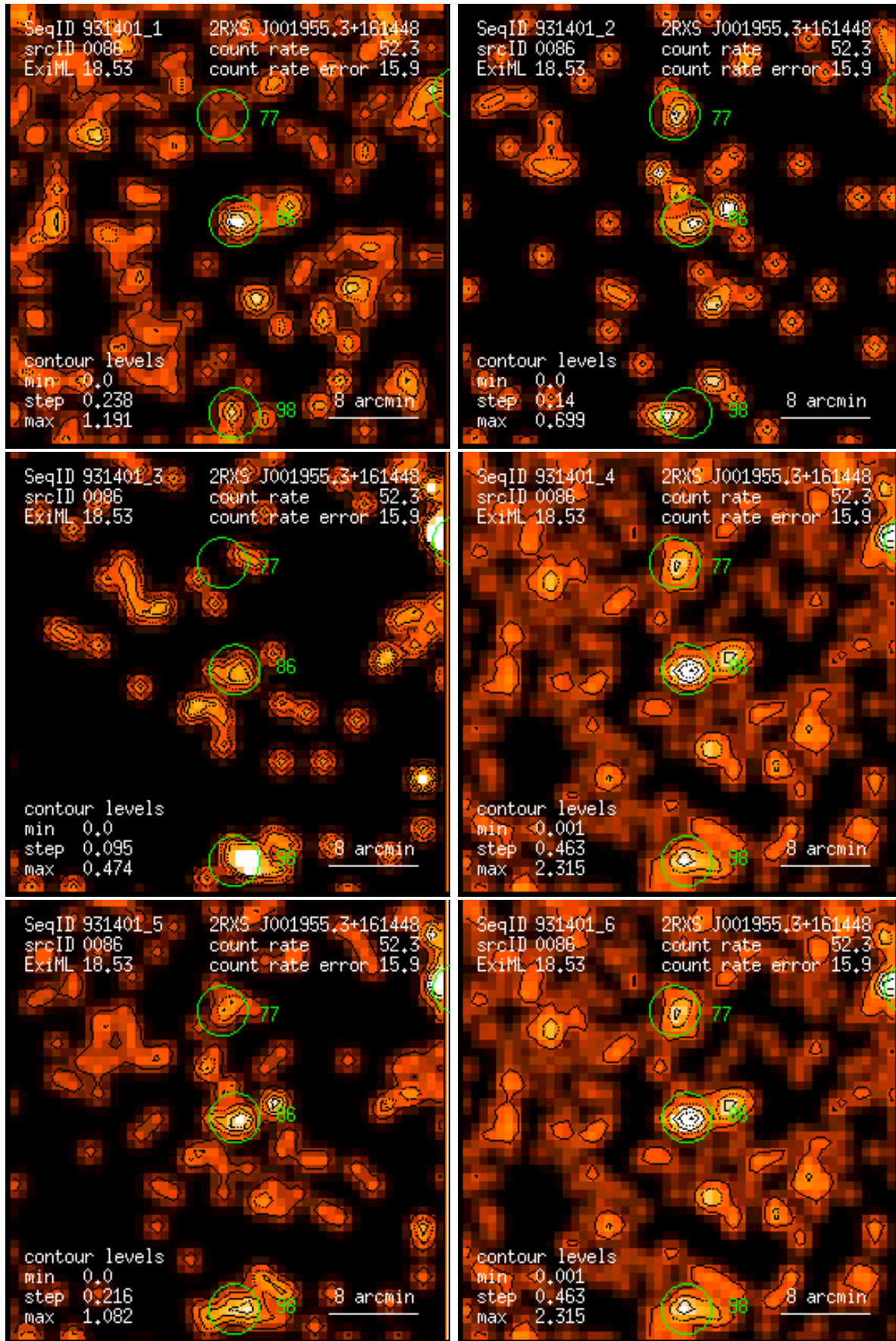
Figure 86: RASS 931401: detection 0086: band rate images, Gaussian filter: (1) PSPC channels 11 – 41, (2) 52 – 90, (3) 91 – 201, (4) 11 – 235, (5) 52 – 201, (6) 11 – 201. Broad band rates in counts/ks. Band rate contour levels in counts/ks/arcmin 2 .
