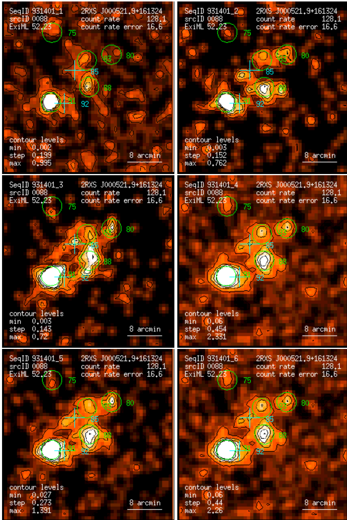
Figure 88: RASS 931401: detection 0088: band rate images, Gaussian filter: (1) PSPC channels 11 – 41, (2) 52 – 90, (3) 91 – 201, (4) 11 – 235, (5) 52 – 201, (6) 11 – 201. Broad band rates in counts/ks. Band rate contour levels in counts/ks/arcmin 2 .
