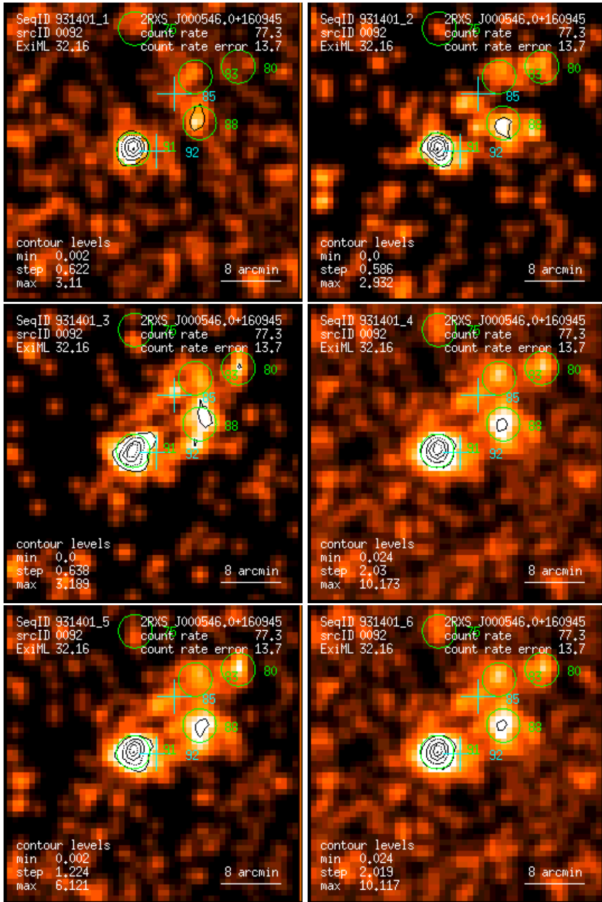
Figure 92: RASS 931401: detection 0092: band rate images, Gaussian filter: (1) PSPC channels 11 – 41, (2) 52 – 90, (3) 91 – 201, (4) 11 – 235, (5) 52 – 201, (6) 11 – 201. Broad band rates in counts/ks. Band rate contour levels in counts/ks/arcmin 2 .
