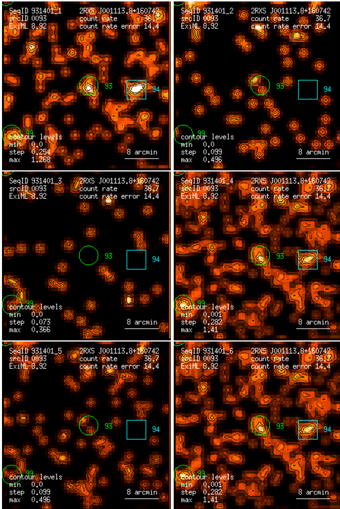
Figure 93: RASS 931401: detection 0093: band rate images, Gaussian filter: (1) PSPC channels 11 – 41, (2) 52 – 90, (3) 91 – 201, (4) 11 – 235, (5) 52 – 201, (6) 11 – 201. Broad band rates in counts/ks. Band rate contour levels in counts/ks/arcmin 2 .
