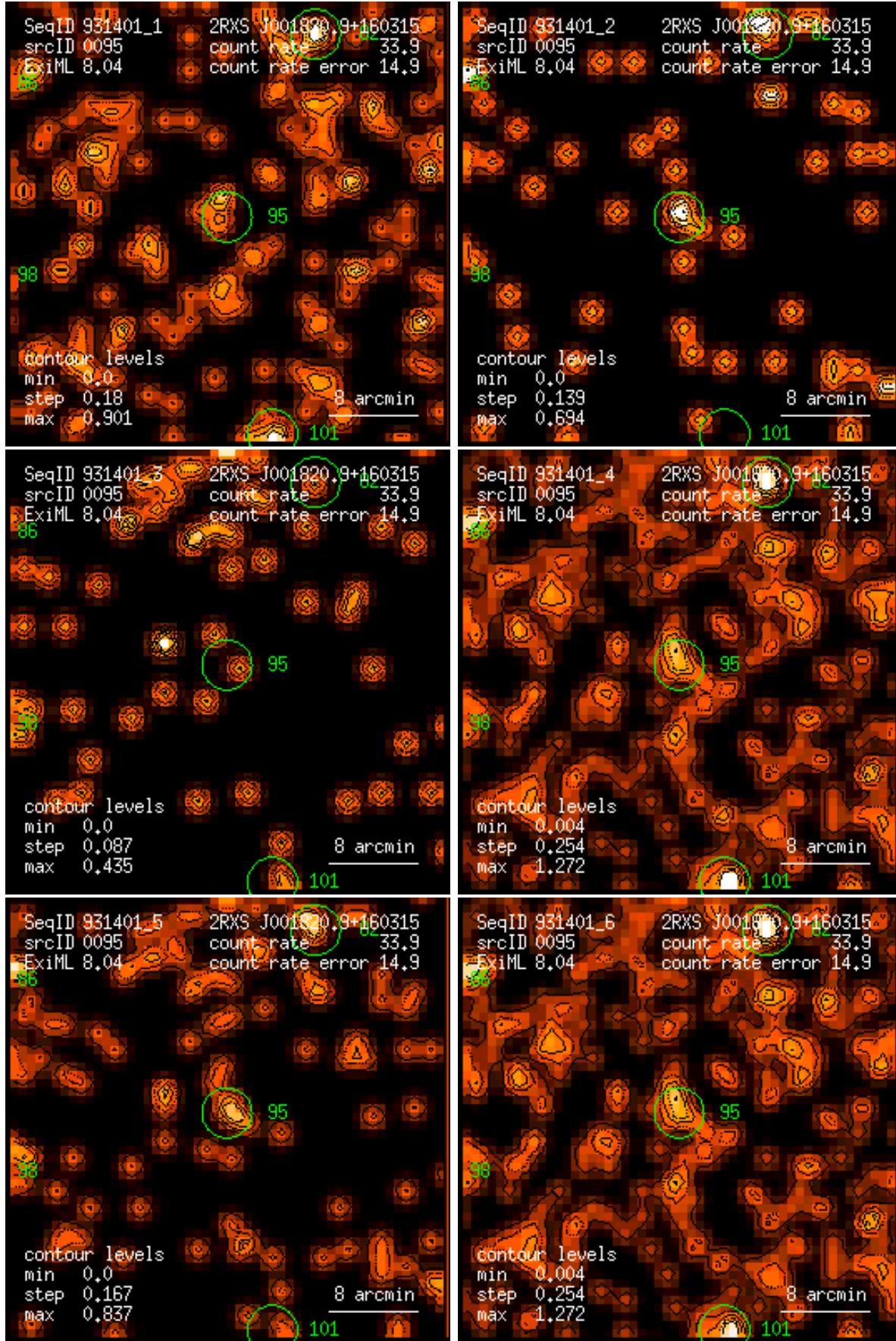
Figure 95: RASS 931401: detection 0095: band rate images, Gaussian filter: (1) PSPC channels 11 – 41, (2) 52 – 90, (3) 91 – 201, (4) 11 – 235, (5) 52 – 201, (6) 11 – 201. Broad band rates in counts/ks. Band rate contour levels in counts/ks/arcmin 2 .
