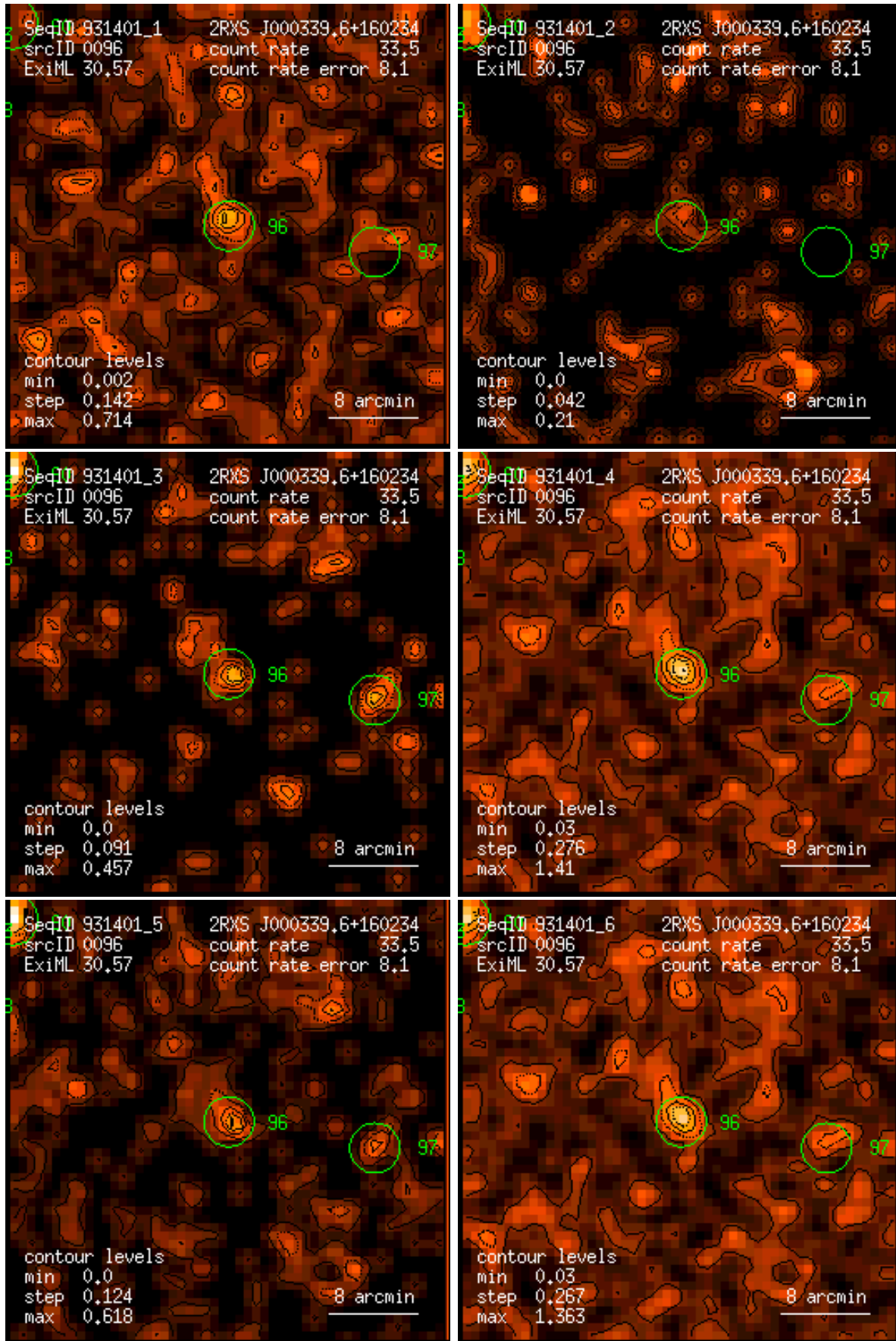
Figure 96: RASS 931401: detection 0096: band rate images, Gaussian filter: (1) PSPC channels 11 – 41, (2) 52 – 90, (3) 91 – 201, (4) 11 – 235, (5) 52 – 201, (6) 11 – 201. Broad band rates in counts/ks. Band rate contour levels in counts/ks/arcmin 2 .
