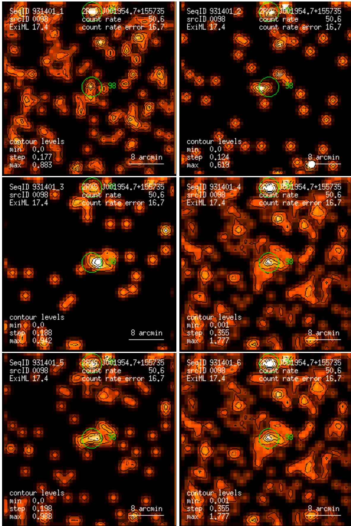
Figure 98: RASS 931401: detection 0098: band rate images, Gaussian filter: (1) PSPC channels 11 – 41, (2) 52 – 90, (3) 91 – 201, (4) 11 – 235, (5) 52 – 201, (6) 11 – 201. Broad band rates in counts/ks. Band rate contour levels in counts/ks/arcmin 2 .
