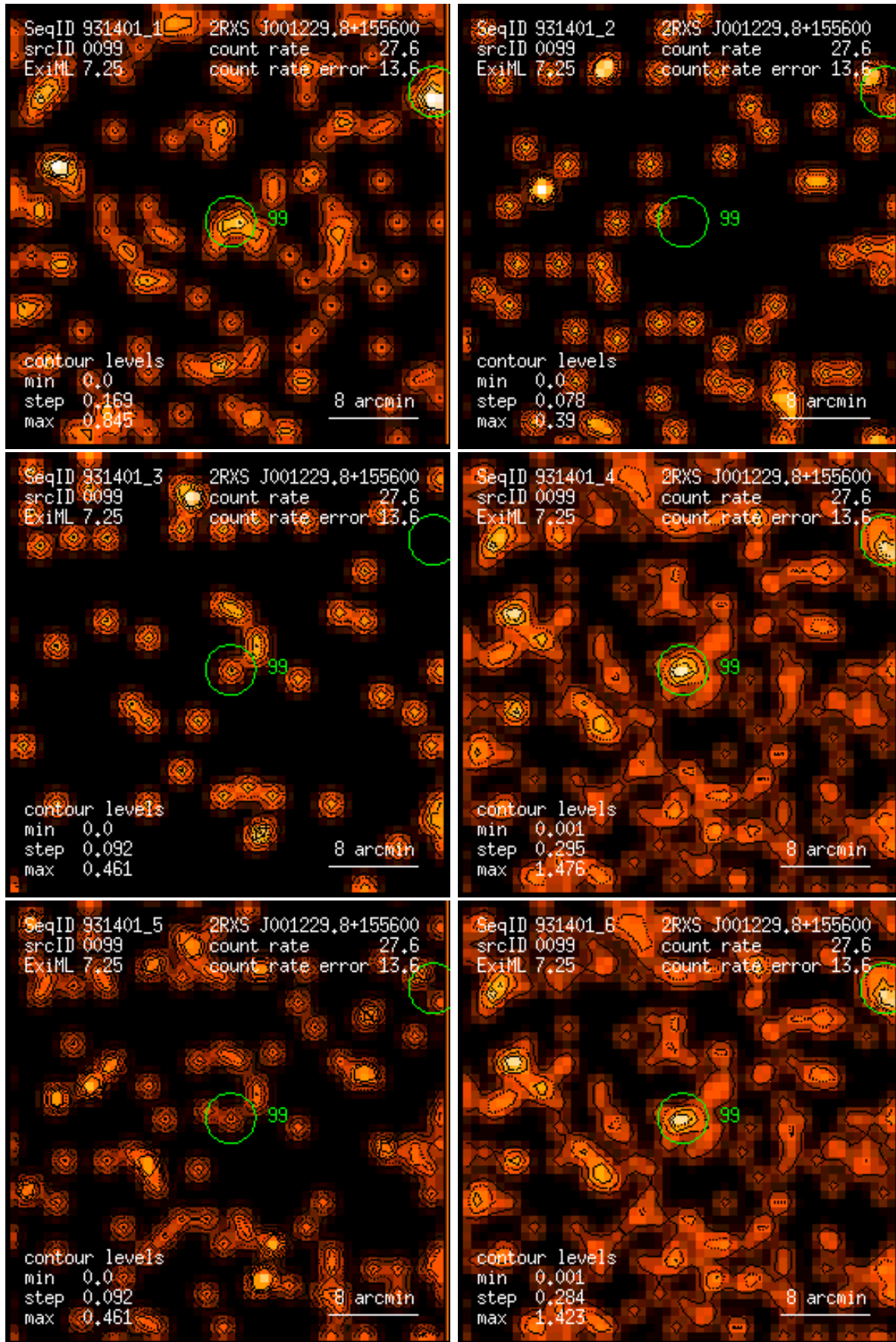
Figure 99: RASS 931401: detection 0099: band rate images, Gaussian filter: (1) PSPC channels 11 – 41, (2) 52 – 90, (3) 91 – 201, (4) 11 – 235, (5) 52 – 201, (6) 11 – 201. Broad band rates in counts/ks. Band rate contour levels in counts/ks/arcmin 2 .
