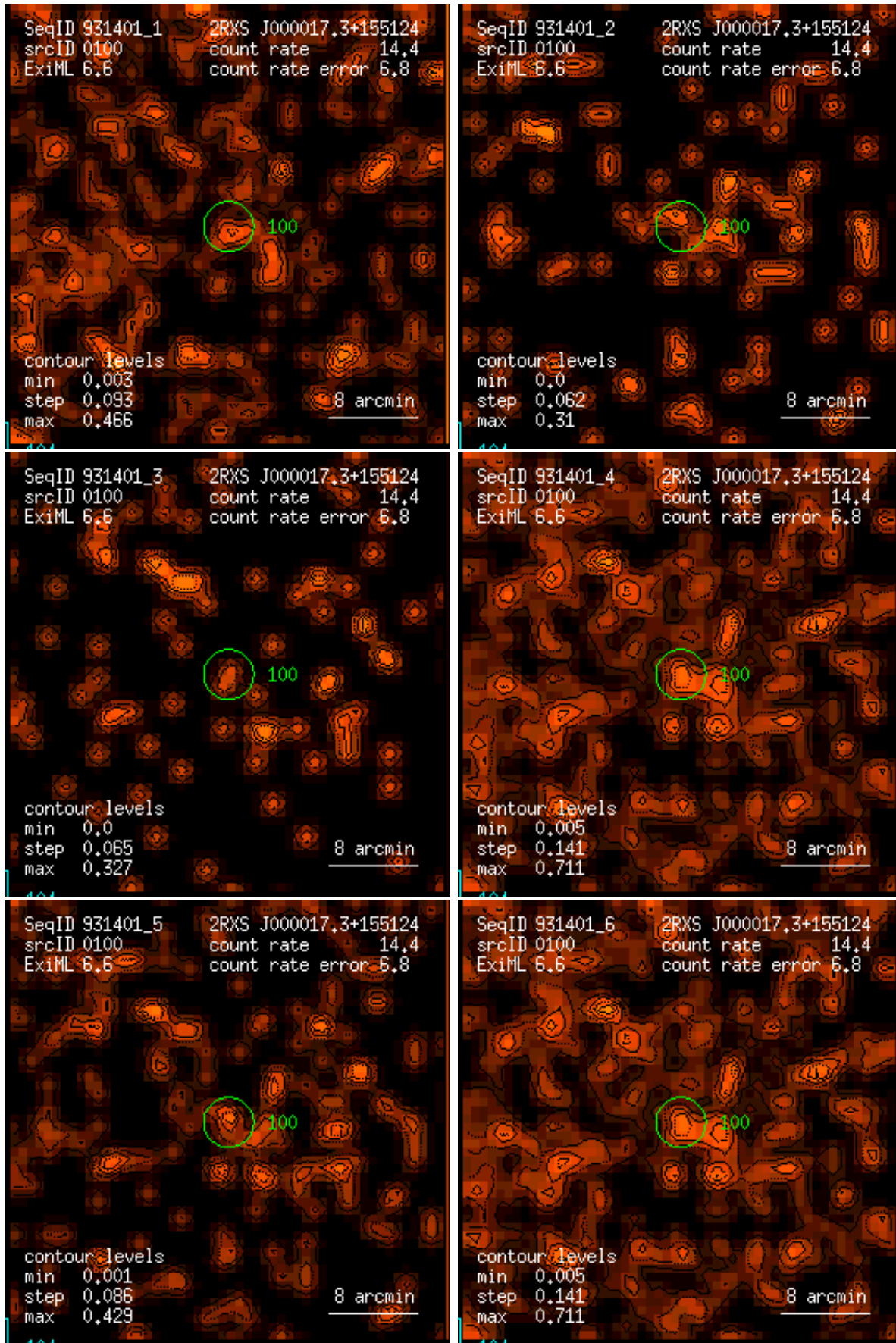
Figure 100: RASS 931401: detection 0100: band rate images, Gaussian filter: (1) PSPC channels 11 – 41, (2) 52 – 90, (3) 91 – 201, (4) 11 – 235, (5) 52 – 201, (6) 11 – 201. Broad band rates in counts/ks. Band rate contour levels in counts/ks/arcmin 2 .
