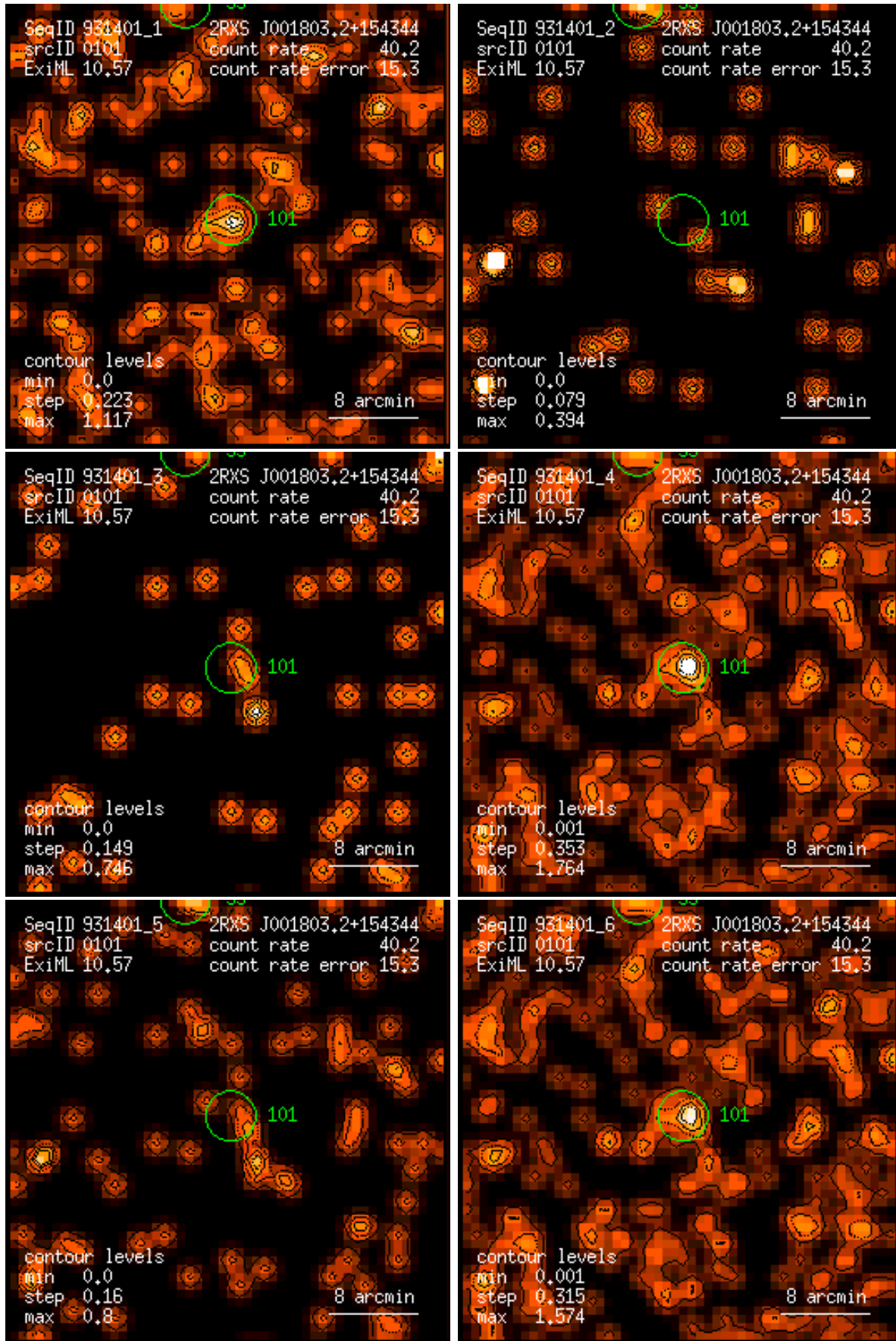
Figure 101: RASS 931401: detection 0101: band rate images, Gaussian filter: (1) PSPC channels 11 – 41, (2) 52 – 90, (3) 91 – 201, (4) 11 – 235, (5) 52 – 201, (6) 11 – 201. Broad band rates in counts/ks. Band rate contour levels in counts/ks/arcmin 2 .
