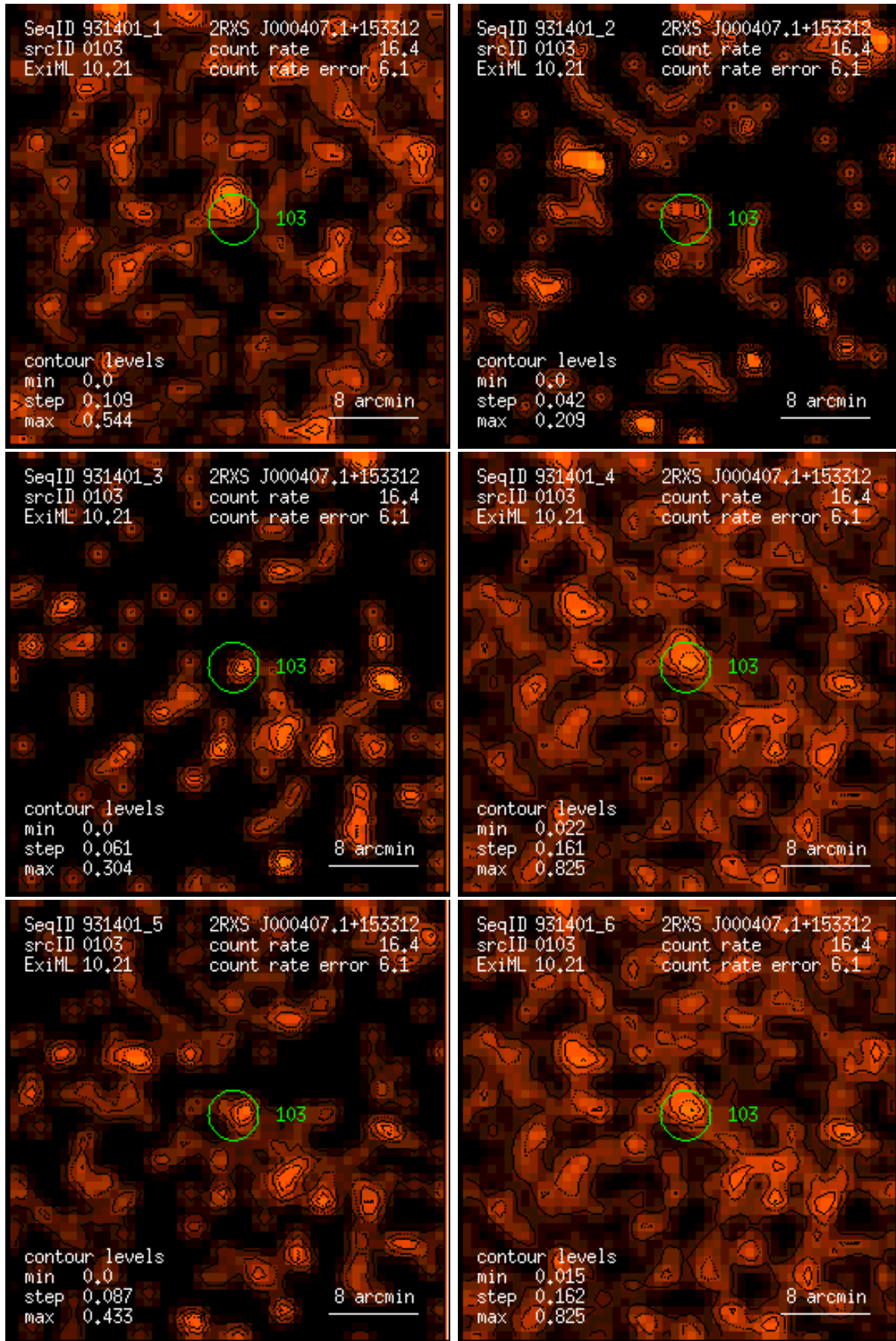
Figure 103: RASS 931401: detection 0103: band rate images, Gaussian filter: (1) PSPC channels 11 – 41, (2) 52 – 90, (3) 91 – 201, (4) 11 – 235, (5) 52 – 201, (6) 11 – 201. Broad band rates in counts/ks. Band rate contour levels in counts/ks/arcmin 2 .
