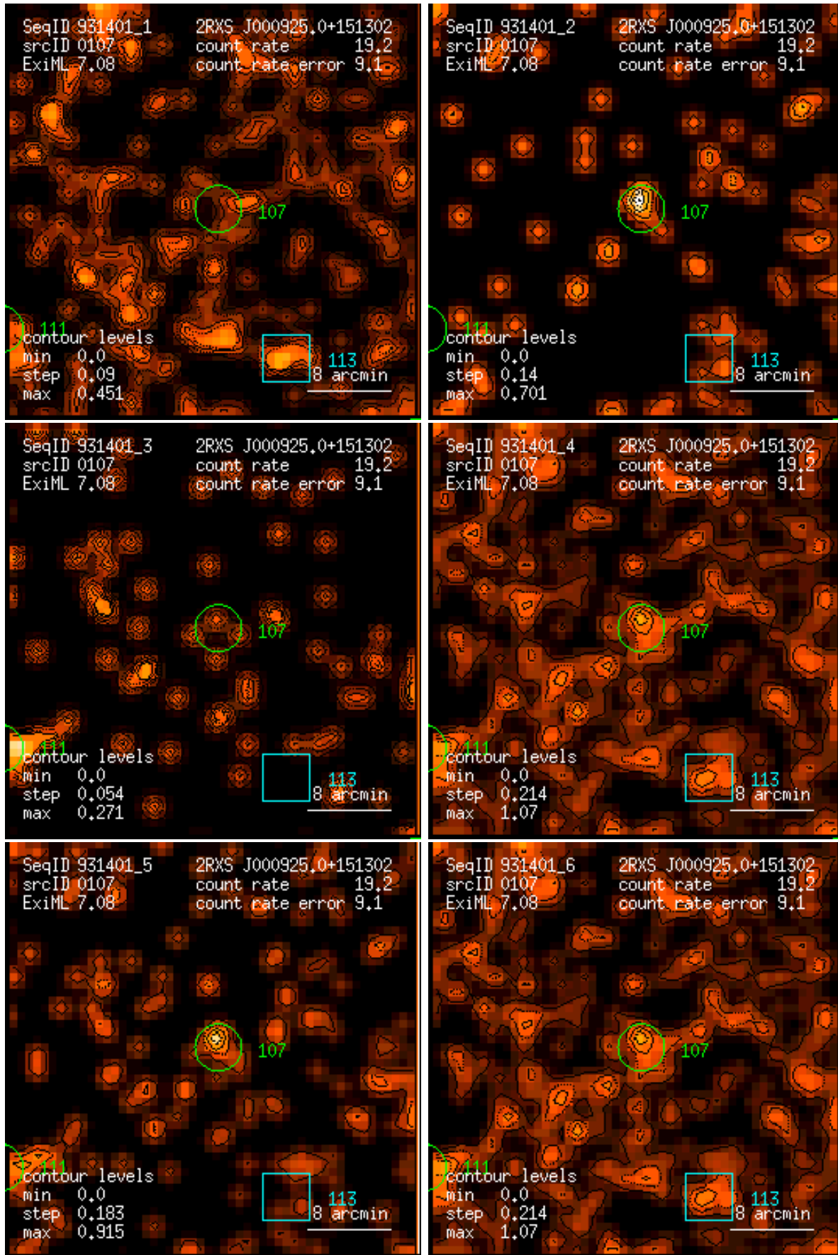
Figure 107: RASS 931401: detection 0107: band rate images, Gaussian filter: (1) PSPC channels 11 – 41, (2) 52 – 90, (3) 91 – 201, (4) 11 – 235, (5) 52 – 201, (6) 11 – 201. Broad band rates in counts/ks. Band rate contour levels in counts/ks/arcmin 2 .
