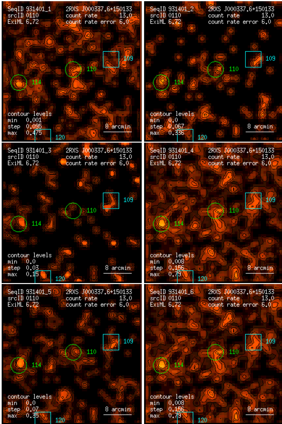
Figure 110: RASS 931401: detection 0110: band rate images, Gaussian filter: (1) PSPC channels 11 – 41, (2) 52 – 90, (3) 91 – 201, (4) 11 – 235, (5) 52 – 201, (6) 11 – 201. Broad band rates in counts/ks. Band rate contour levels in counts/ks/arcmin 2 .
