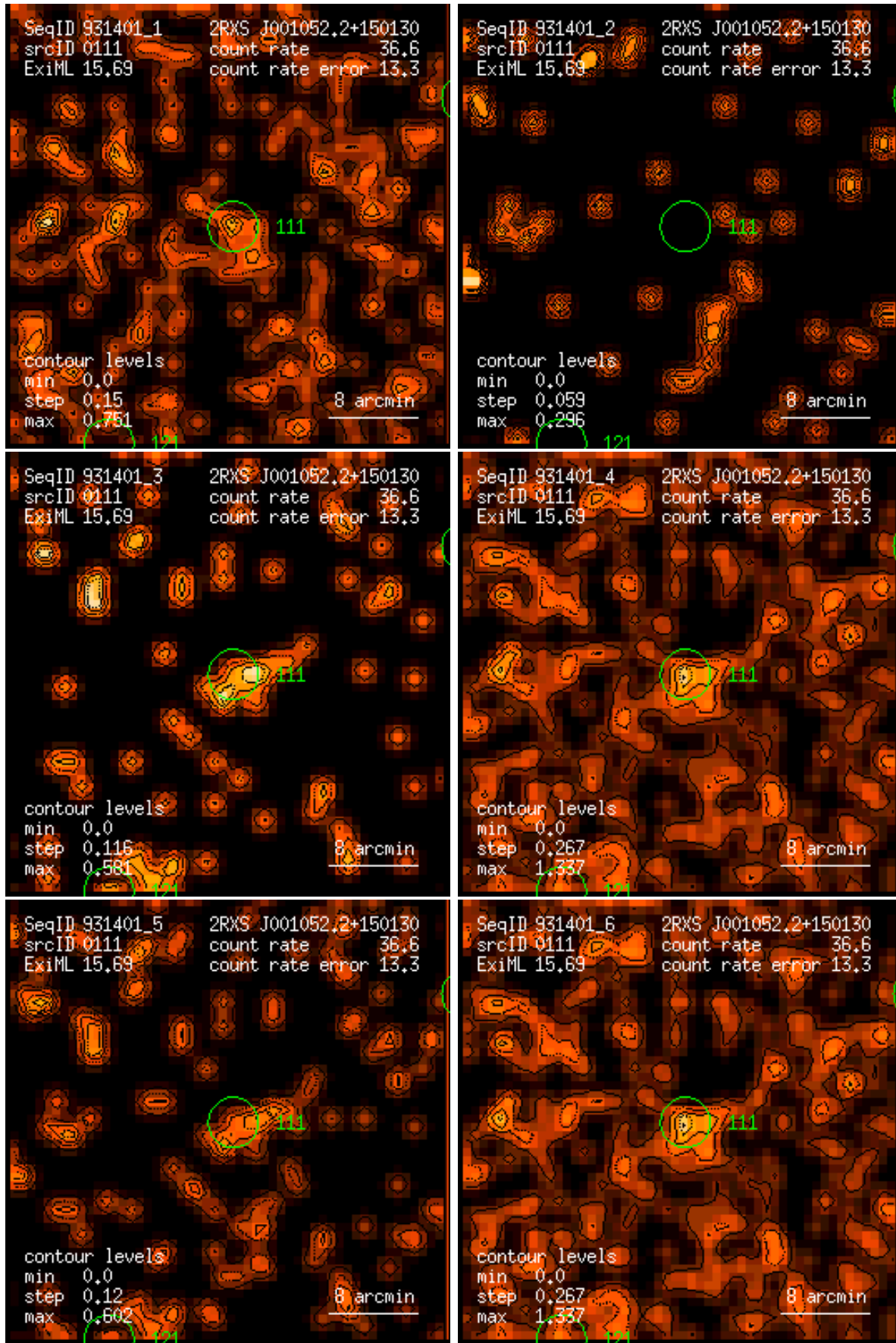
Figure 111: RASS 931401: detection 0111: band rate images, Gaussian filter: (1) PSPC channels 11 – 41, (2) 52 – 90, (3) 91 – 201, (4) 11 – 235, (5) 52 – 201, (6) 11 – 201. Broad band rates in counts/ks. Band rate contour levels in counts/ks/arcmin 2 .
