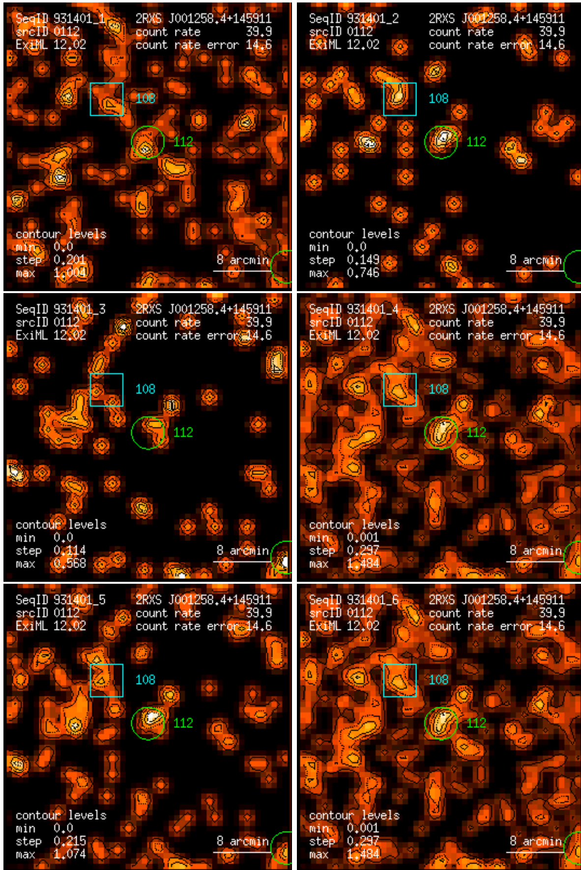
Figure 112: RASS 931401: detection 0112: band rate images, Gaussian filter: (1) PSPC channels 11 – 41, (2) 52 – 90, (3) 91 – 201, (4) 11 – 235, (5) 52 – 201, (6) 11 – 201. Broad band rates in counts/ks. Band rate contour levels in counts/ks/arcmin 2 .
