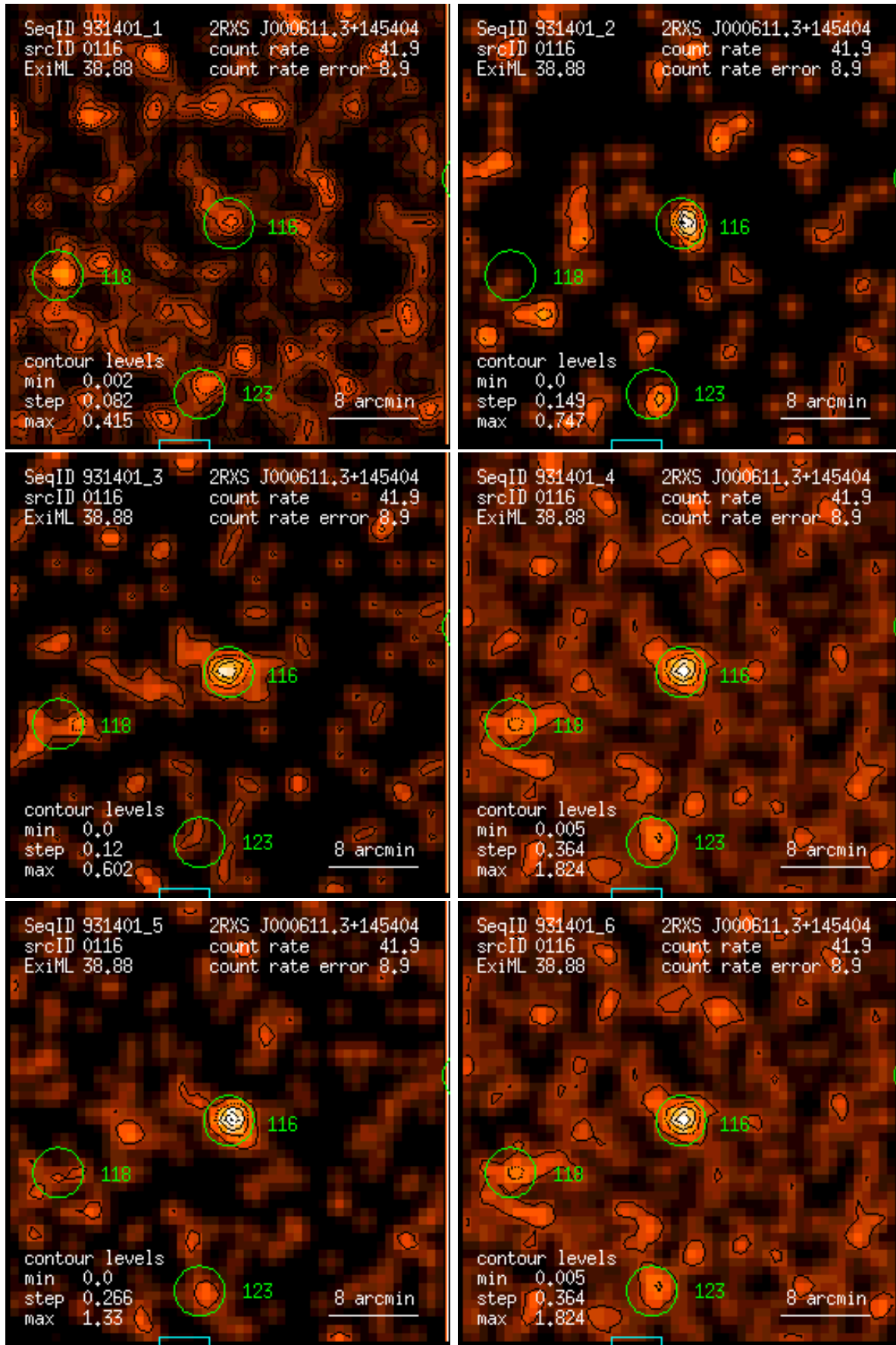
Figure 116: RASS 931401: detection 0116: band rate images, Gaussian filter: (1) PSPC channels 11 – 41, (2) 52 – 90, (3) 91 – 201, (4) 11 – 235, (5) 52 – 201, (6) 11 – 201. Broad band rates in counts/ks. Band rate contour levels in counts/ks/arcmin 2 .
