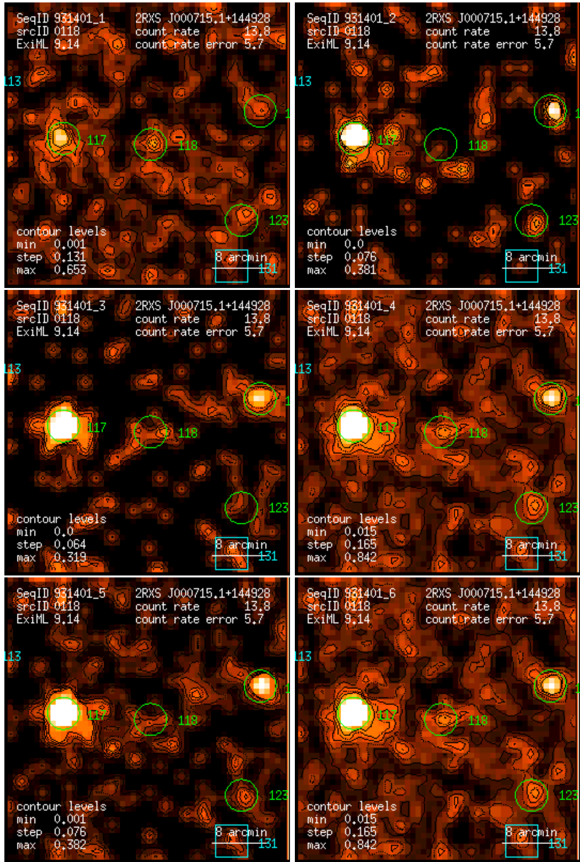
Figure 118: RASS 931401: detection 0118: band rate images, Gaussian filter: (1) PSPC channels 11 – 41, (2) 52 – 90, (3) 91 – 201, (4) 11 – 235, (5) 52 – 201, (6) 11 – 201. Broad band rates in counts/ks. Band rate contour levels in counts/ks/arcmin 2 .
