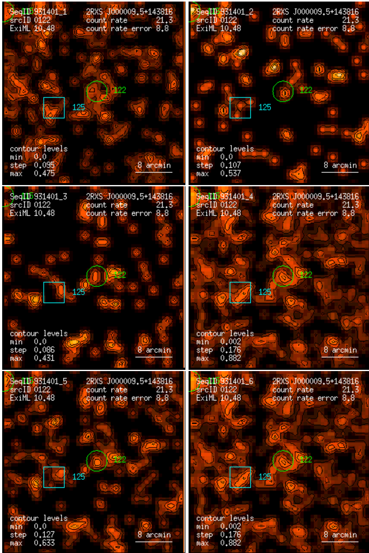
Figure 122: RASS 931401: detection 0122: band rate images, Gaussian filter: (1) PSPC channels 11 – 41, (2) 52 – 90, (3) 91 – 201, (4) 11 – 235, (5) 52 – 201, (6) 11 – 201. Broad band rates in counts/ks. Band rate contour levels in counts/ks/arcmin 2 .
