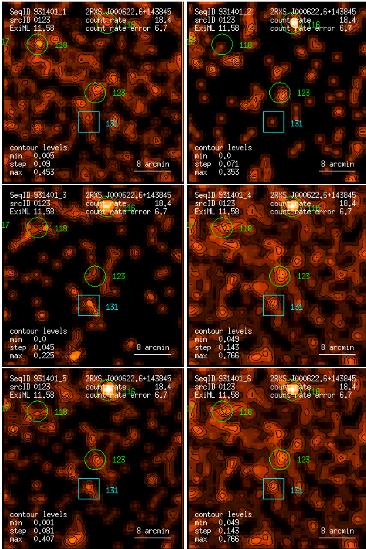
Figure 123: RASS 931401: detection 0123: band rate images, Gaussian filter: (1) PSPC channels 11 – 41, (2) 52 – 90, (3) 91 – 201, (4) 11 – 235, (5) 52 – 201, (6) 11 – 201. Broad band rates in counts/ks. Band rate contour levels in counts/ks/arcmin 2 .
