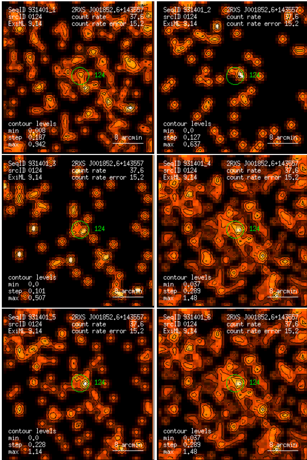
Figure 124: RASS 931401: detection 0124: band rate images, Gaussian filter: (1) PSPC channels 11 – 41, (2) 52 – 90, (3) 91 – 201, (4) 11 – 235, (5) 52 – 201, (6) 11 – 201. Broad band rates in counts/ks. Band rate contour levels in counts/ks/arcmin 2 .
