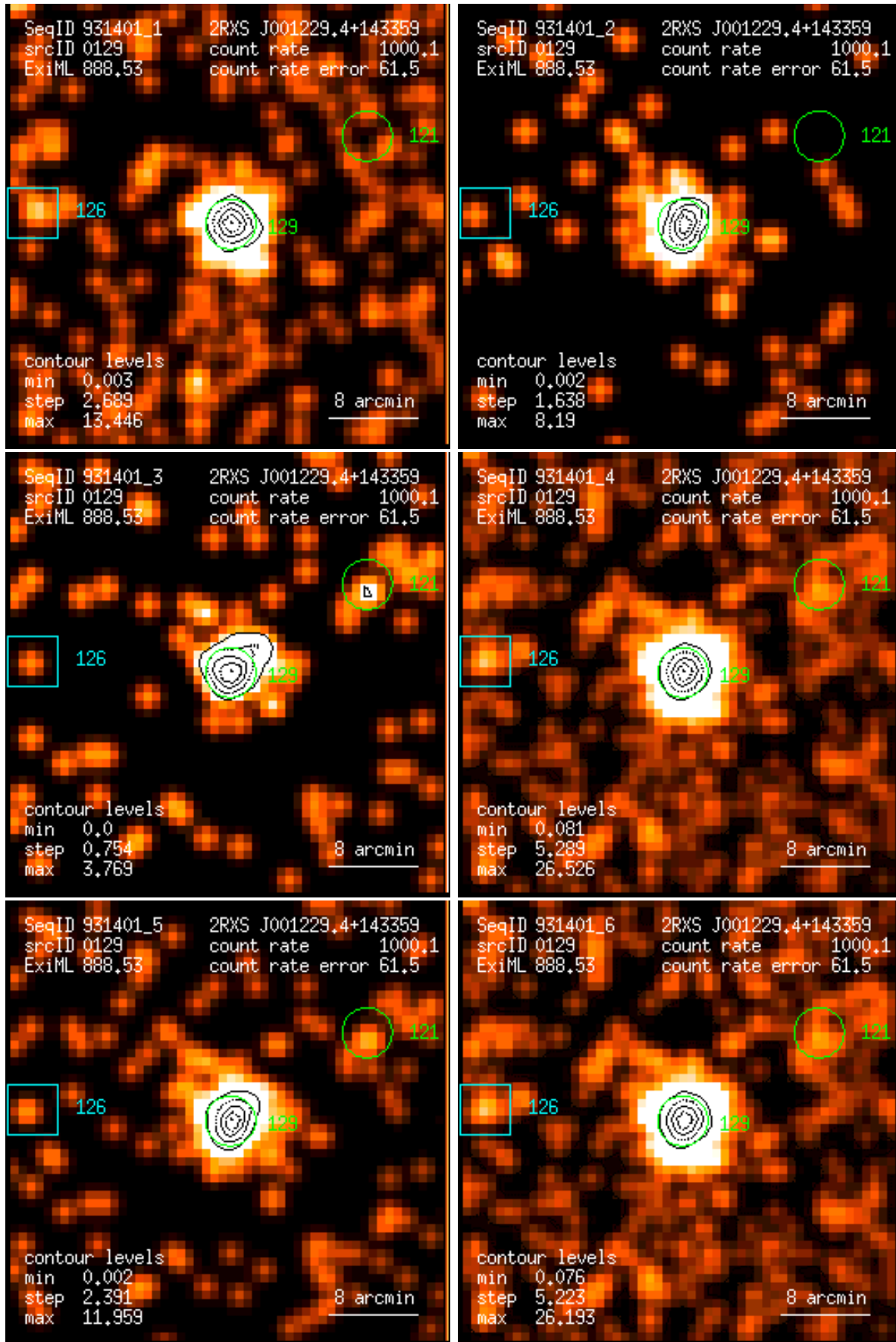
Figure 129: RASS 931401: detection 0129: band rate images, Gaussian filter: (1) PSPC channels 11 – 41, (2) 52 – 90, (3) 91 – 201, (4) 11 – 235, (5) 52 – 201, (6) 11 – 201. Broad band rates in counts/ks. Band rate contour levels in counts/ks/arcmin 2 .
