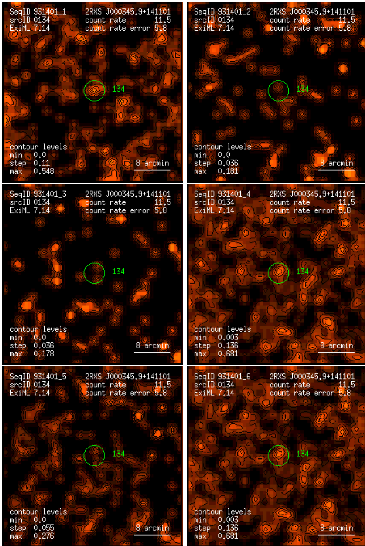
Figure 134: RASS 931401: detection 0134: band rate images, Gaussian filter: (1) PSPC channels 11 – 41, (2) 52 – 90, (3) 91 – 201, (4) 11 – 235, (5) 52 – 201, (6) 11 – 201. Broad band rates in counts/ks. Band rate contour levels in counts/ks/arcmin 2 .
