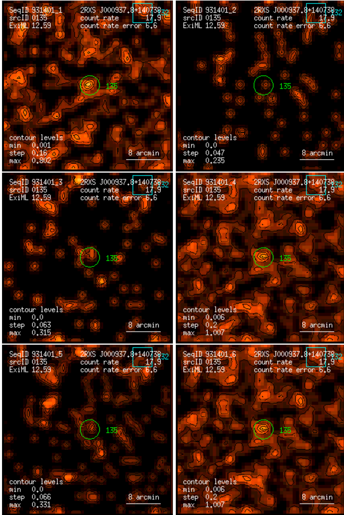
Figure 135: RASS 931401: detection 0135: band rate images, Gaussian filter: (1) PSPC channels 11 – 41, (2) 52 – 90, (3) 91 – 201, (4) 11 – 235, (5) 52 – 201, (6) 11 – 201. Broad band rates in counts/ks. Band rate contour levels in counts/ks/arcmin 2 .
