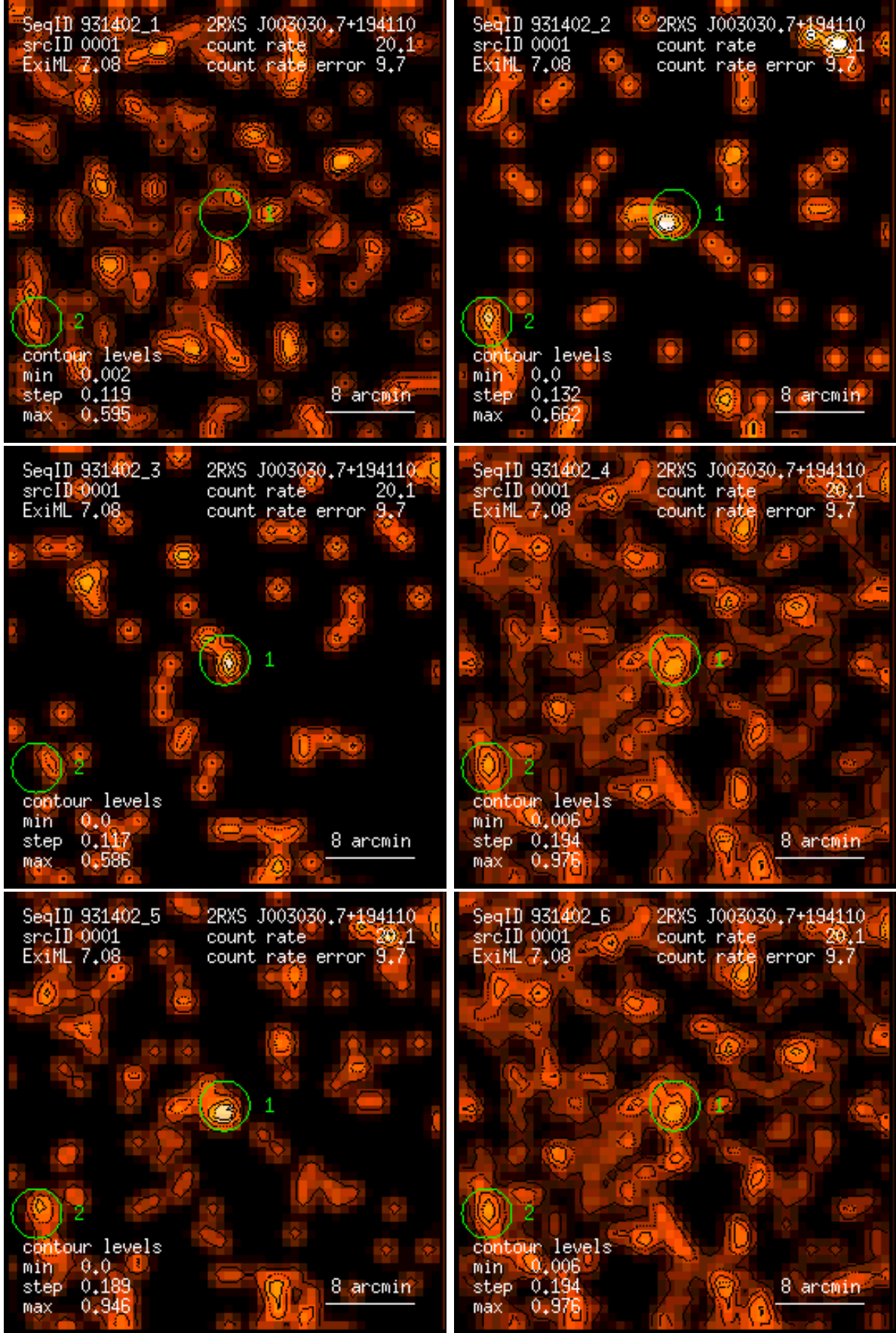
Figure 1: RASS 931402: detection 0001: band rate images, Gaussian filter: (1) PSPC channels 11 – 41, (2) 52 – 90, (3) 91 – 201, (4) 11 – 235, (5) 52 – 201, (6) 11 – 201. Broad band rates in counts/ks. Band rate contour levels in counts/ks/arcmin 2 .
