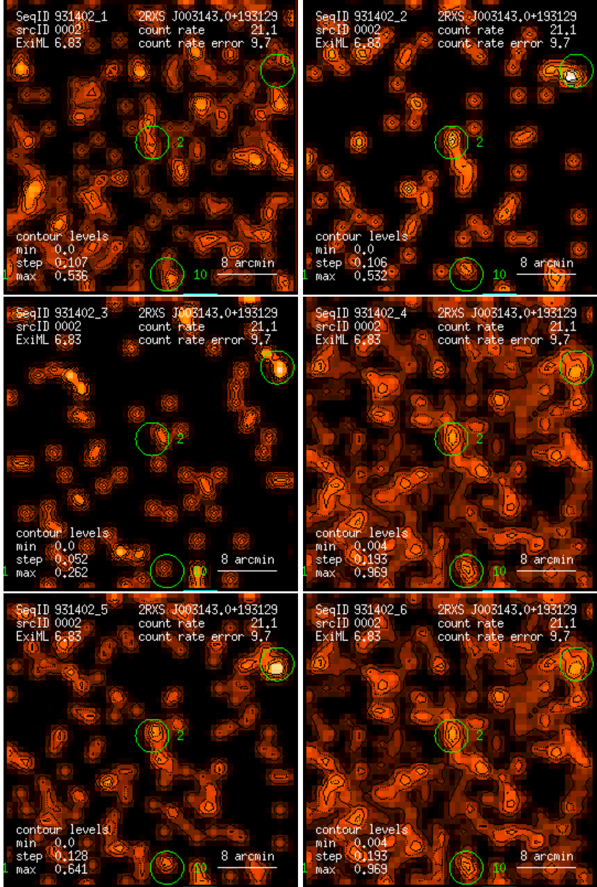
Figure 2: RASS 931402: detection 0002: band rate images, Gaussian filter: (1) PSPC channels 11 – 41, (2) 52 – 90, (3) 91 – 201, (4) 11 – 235, (5) 52 – 201, (6) 11 – 201. Broad band rates in counts/ks. Band rate contour levels in counts/ks/arcmin 2 .
