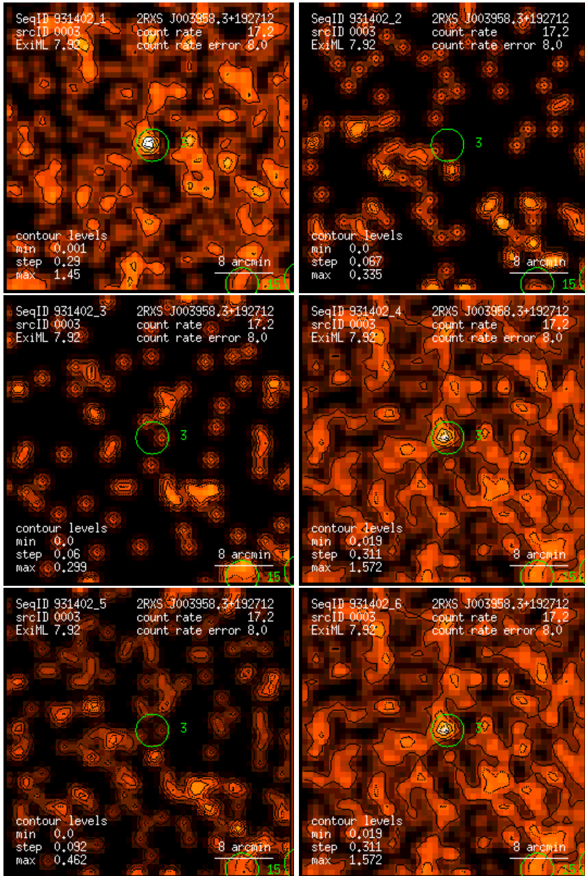
Figure 3: RASS 931402: detection 0003: band rate images, Gaussian filter: (1) PSPC channels 11 – 41, (2) 52 – 90, (3) 91 – 201, (4) 11 – 235, (5) 52 – 201, (6) 11 – 201. Broad band rates in counts/ks. Band rate contour levels in counts/ks/arcmin 2 .
