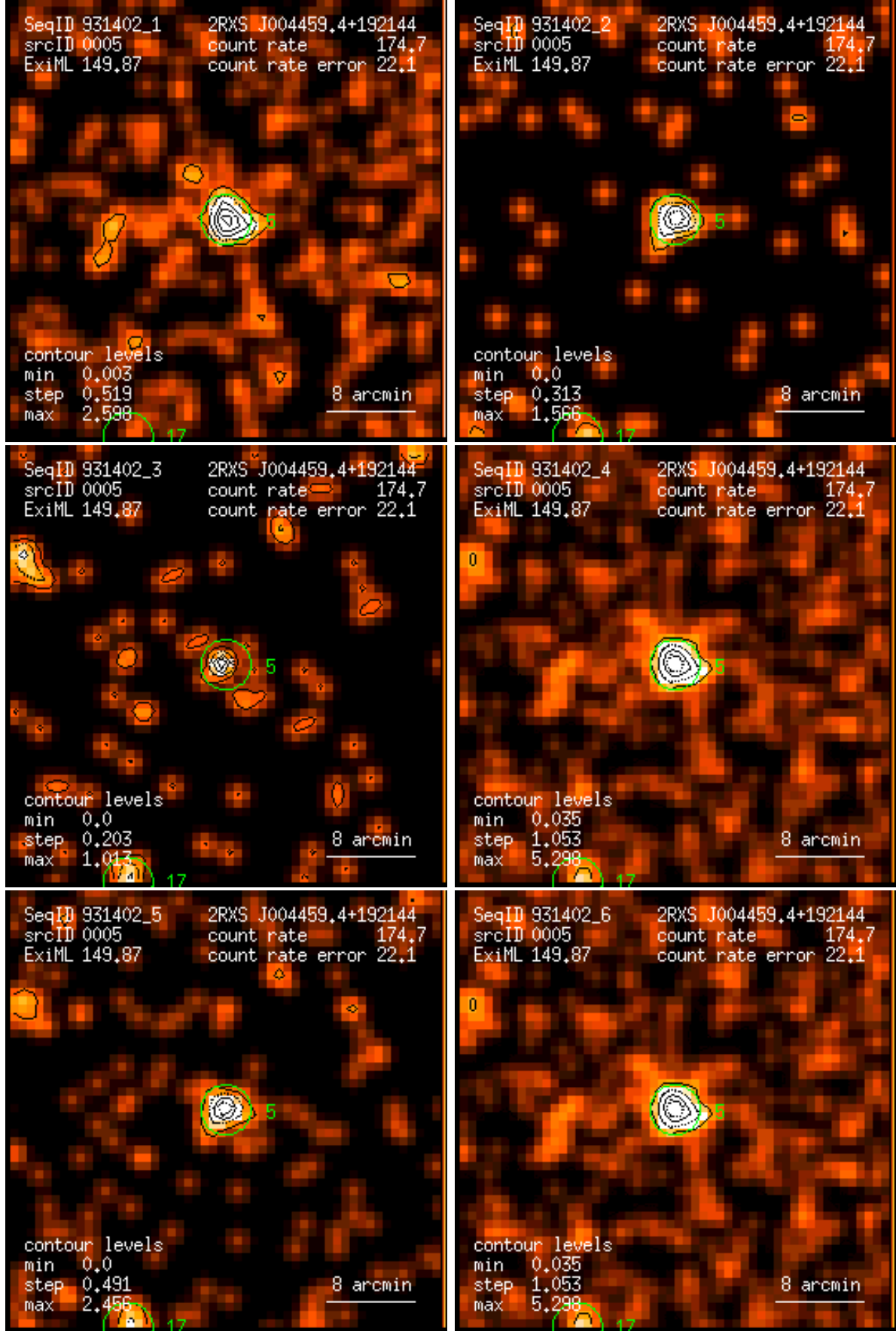
Figure 5: RASS 931402: detection 0005: band rate images, Gaussian filter: (1) PSPC channels 11 – 41, (2) 52 – 90, (3) 91 – 201, (4) 11 – 235, (5) 52 – 201, (6) 11 – 201. Broad band rates in counts/ks. Band rate contour levels in counts/ks/arcmin 2 .
