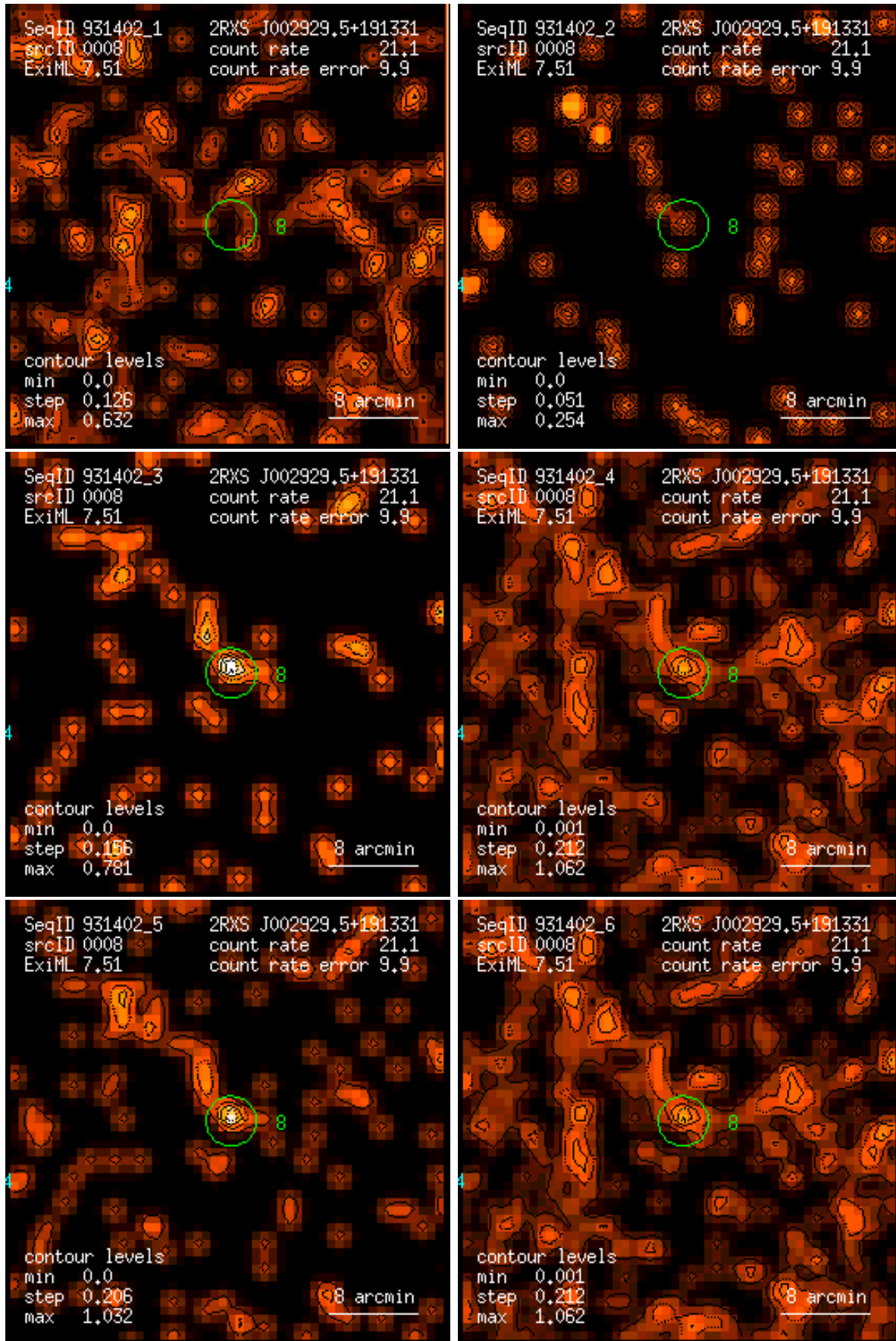
Figure 8: RASS 931402: detection 0008: band rate images, Gaussian filter: (1) PSPC channels 11 – 41, (2) 52 – 90, (3) 91 – 201, (4) 11 – 235, (5) 52 – 201, (6) 11 – 201. Broad band rates in counts/ks. Band rate contour levels in counts/ks/arcmin 2 .
